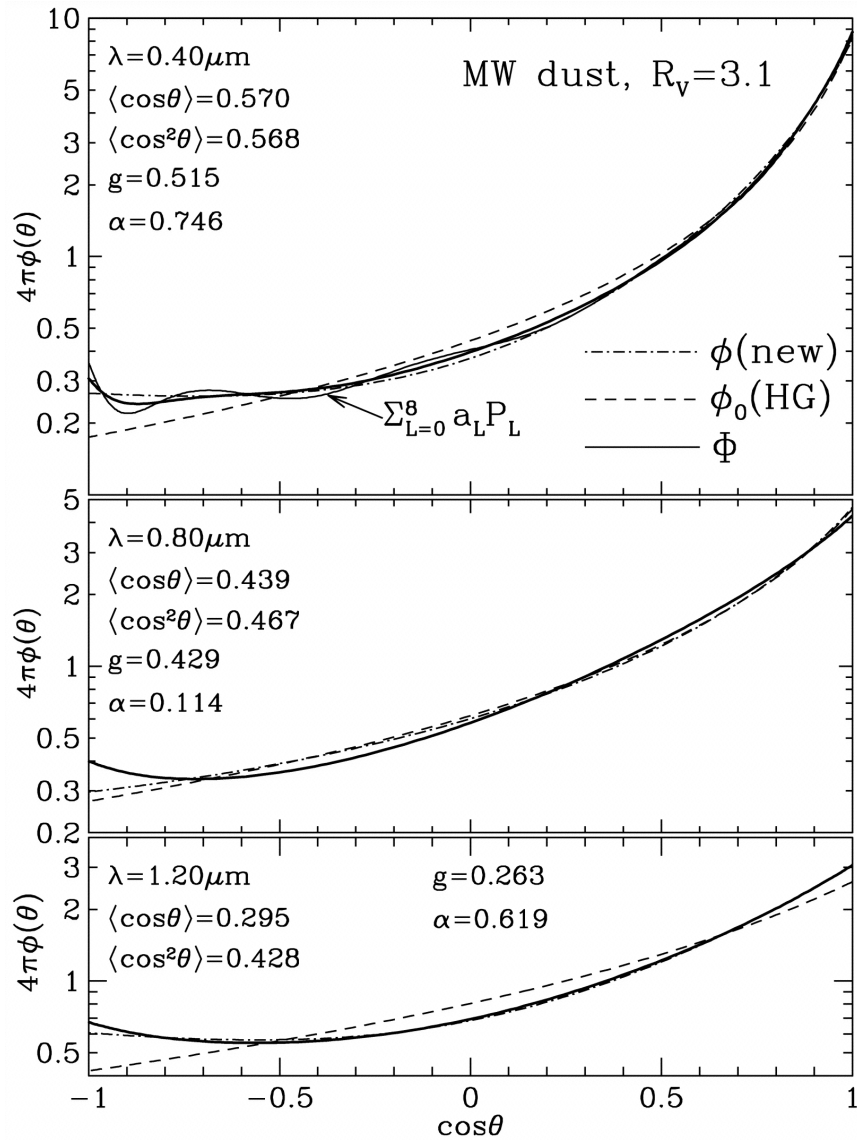
Fig. 6. from Scattering by Interstellar Dust Grains. I. Optical and Ultraviolet Draine 2003 ApJ 598 1017 doi:10.1086/379118 https://dx.doi.org/10.1086/379118 © 2003. The American Astronomical Society. All rights reserved. Printed in U.S.A.
