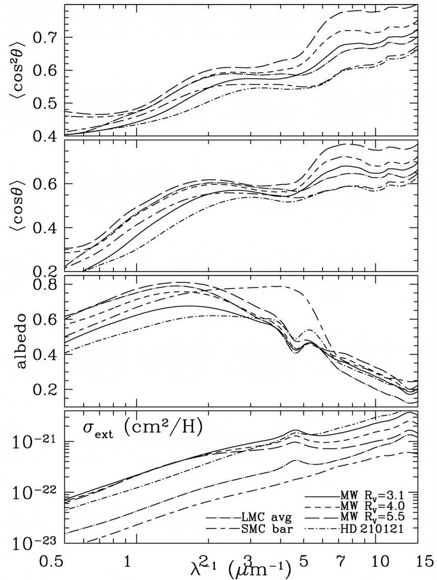
Fig. 4. from Scattering by Interstellar Dust Grains. I. Optical and Ultraviolet Draine 2003 ApJ 598 1017 doi:10.1086/379118 https://dx.doi.org/10.1086/379118 © 2003. The American Astronomical Society. All rights reserved. Printed in U.S.A.
