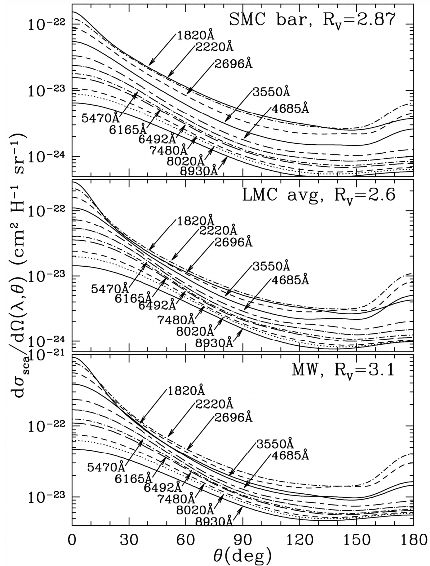
Fig. 3. from Scattering by Interstellar Dust Grains. I. Optical and Ultraviolet Draine 2003 ApJ 598 1017 doi:10.1086/379118 https://dx.doi.org/10.1086/379118 © 2003. The American Astronomical Society. All rights reserved. Printed in U.S.A.
