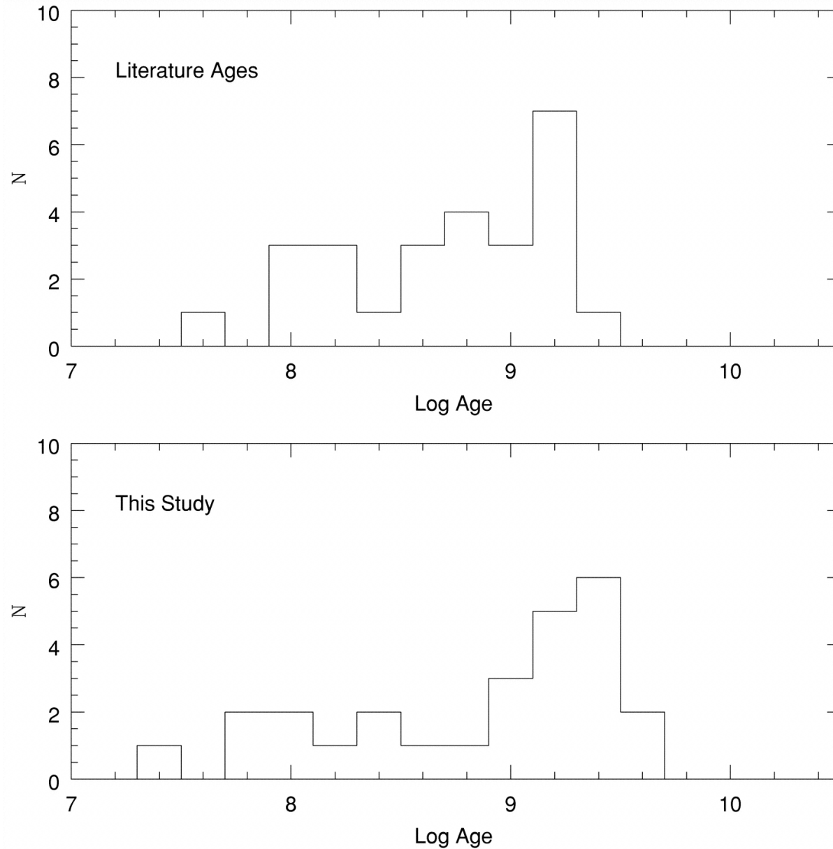
Fig. 24. from Analyzing Starbursts Using Magellanic Cloud Star Clusters as Simple Stellar Populations Leonardi & Rose 2003 AJ 126 1811 doi:10.1086/377617 https://dx.doi.org/10.1086/377617 © 2003. The American Astronomical Society. All rights reserved. Printed in U.S.A.
