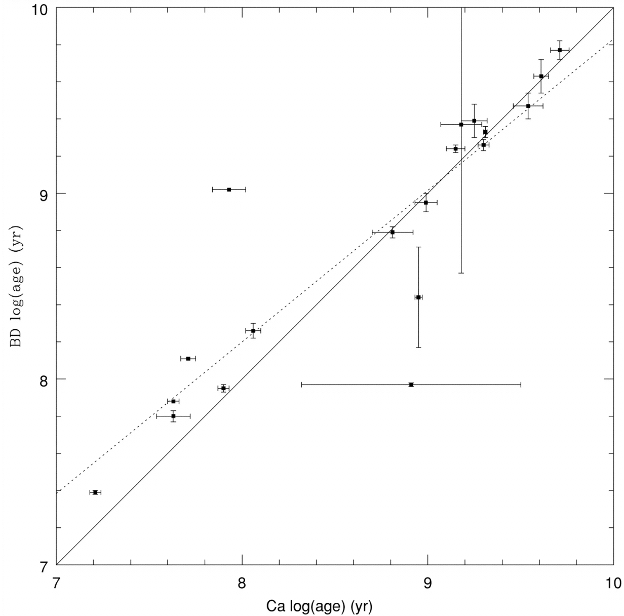
Fig. 21. from Analyzing Starbursts Using Magellanic Cloud Star Clusters as Simple Stellar Populations Leonardi & Rose 2003 AJ 126 1811 doi:10.1086/377617 https://dx.doi.org/10.1086/377617 © 2003. The American Astronomical Society. All rights reserved. Printed in U.S.A.
