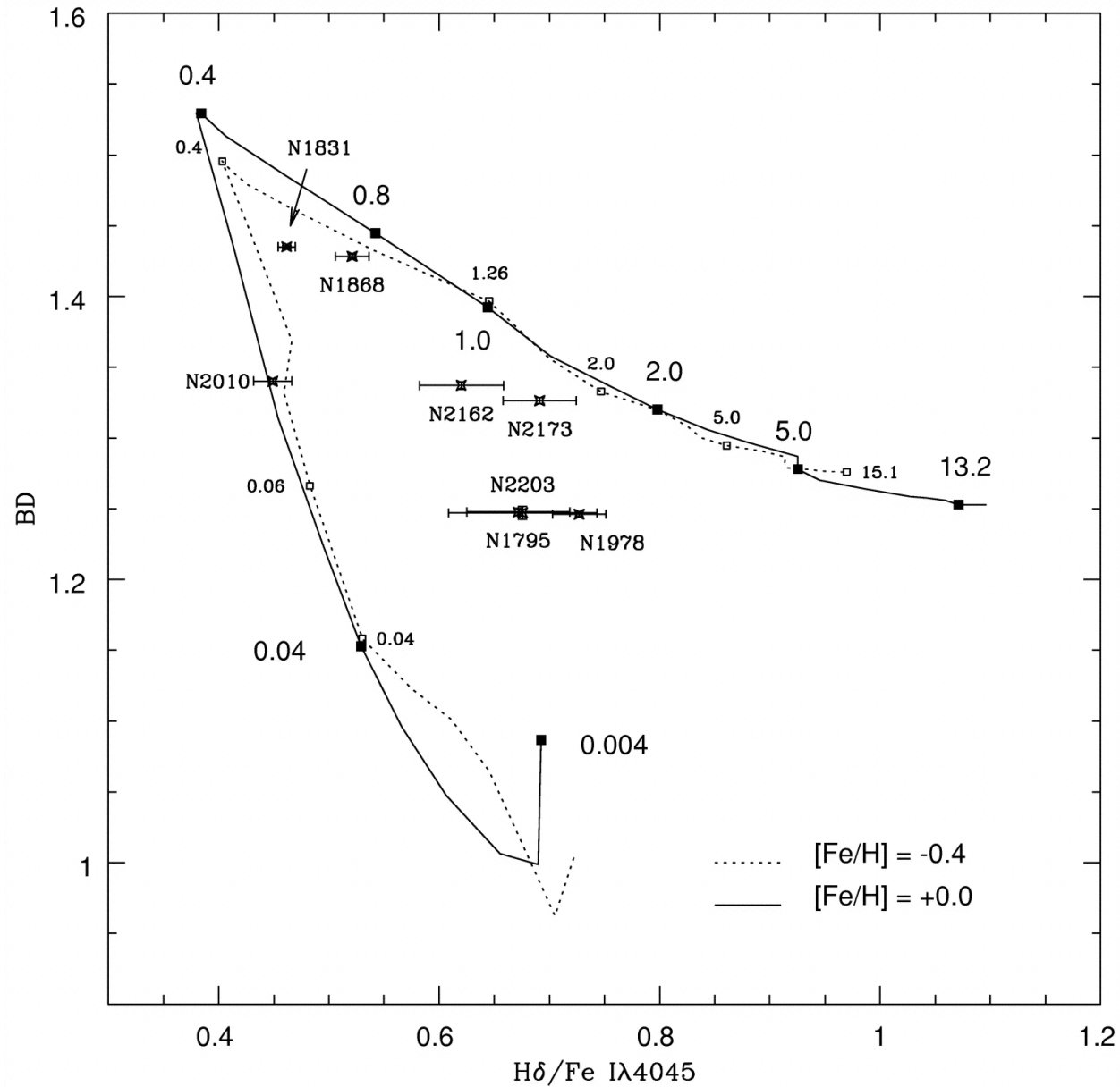
Fig. 20. from Analyzing Starbursts Using Magellanic Cloud Star Clusters as Simple Stellar Populations Leonardi & Rose 2003 AJ 126 1811 doi:10.1086/377617 https://dx.doi.org/10.1086/377617 © 2003. The American Astronomical Society. All rights reserved. Printed in U.S.A.
