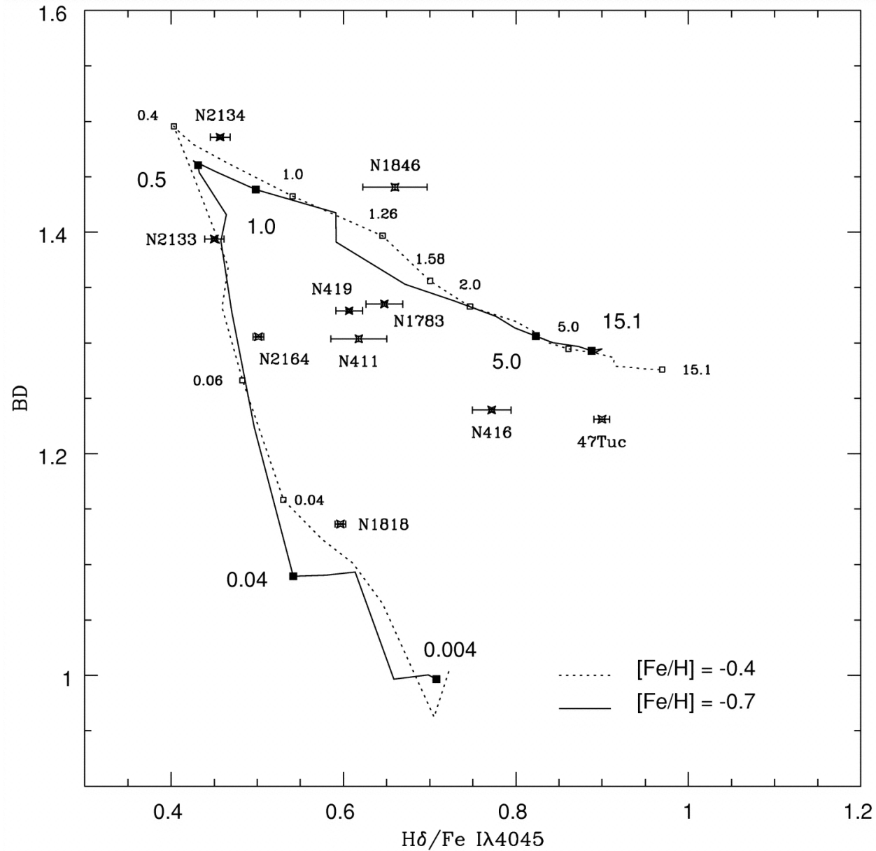
Fig. 18. from Analyzing Starbursts Using Magellanic Cloud Star Clusters as Simple Stellar Populations Leonardi & Rose 2003 AJ 126 1811 doi:10.1086/377617 https://dx.doi.org/10.1086/377617 © 2003. The American Astronomical Society. All rights reserved. Printed in U.S.A.
