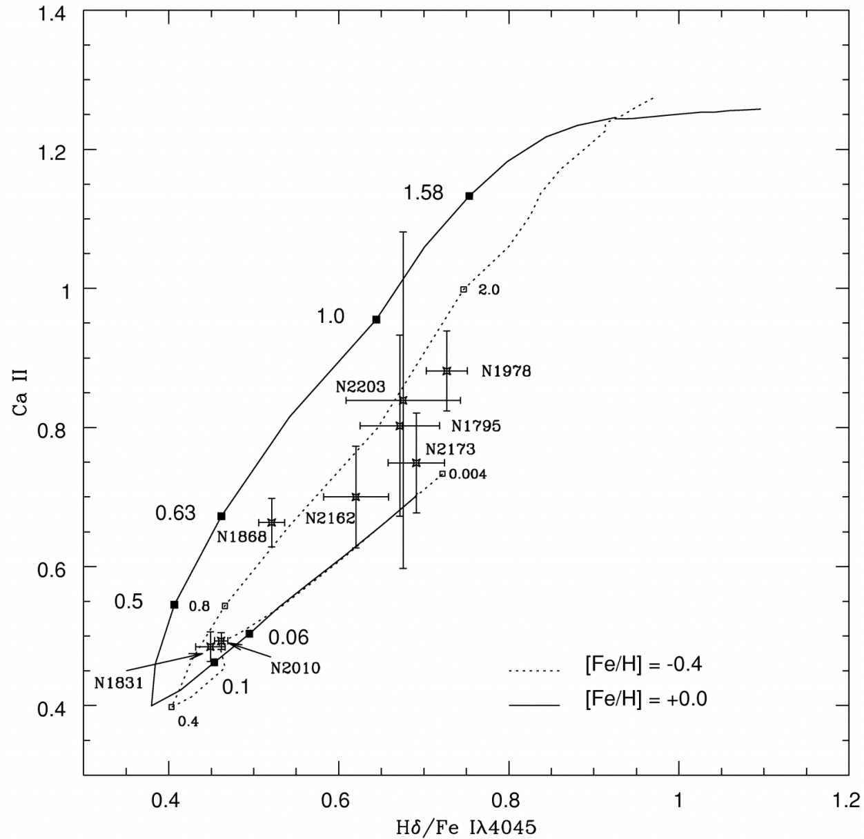
Fig. 15. from Analyzing Starbursts Using Magellanic Cloud Star Clusters as Simple Stellar Populations Leonardi & Rose 2003 AJ 126 1811 doi:10.1086/377617 https://dx.doi.org/10.1086/377617
