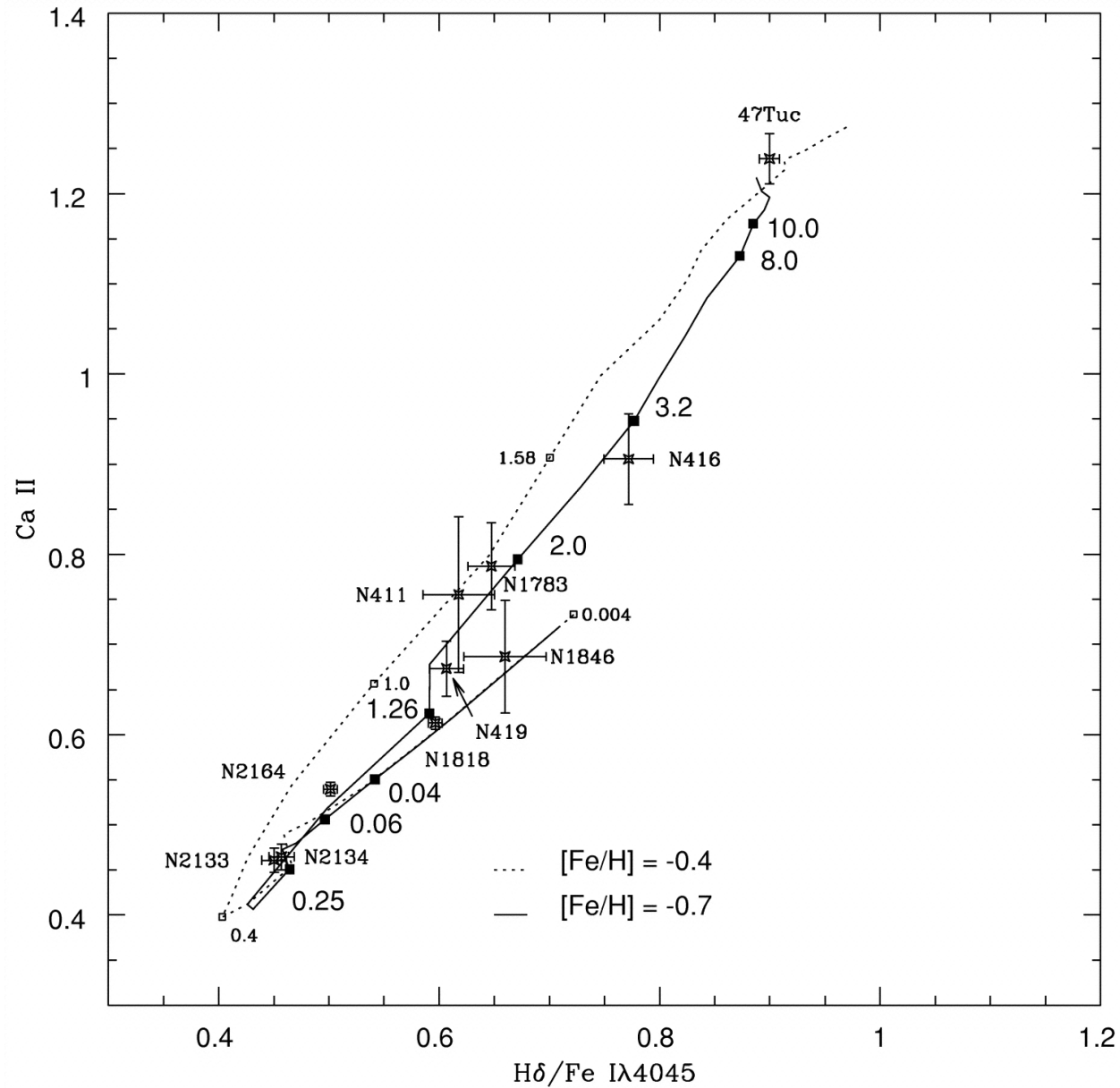
Fig. 13. from Analyzing Starbursts Using Magellanic Cloud Star Clusters as Simple Stellar Populations Leonardi & Rose 2003 AJ 126 1811 doi:10.1086/377617 https://dx.doi.org/10.1086/377617 © 2003. The American Astronomical Society. All rights reserved. Printed in U.S.A.
