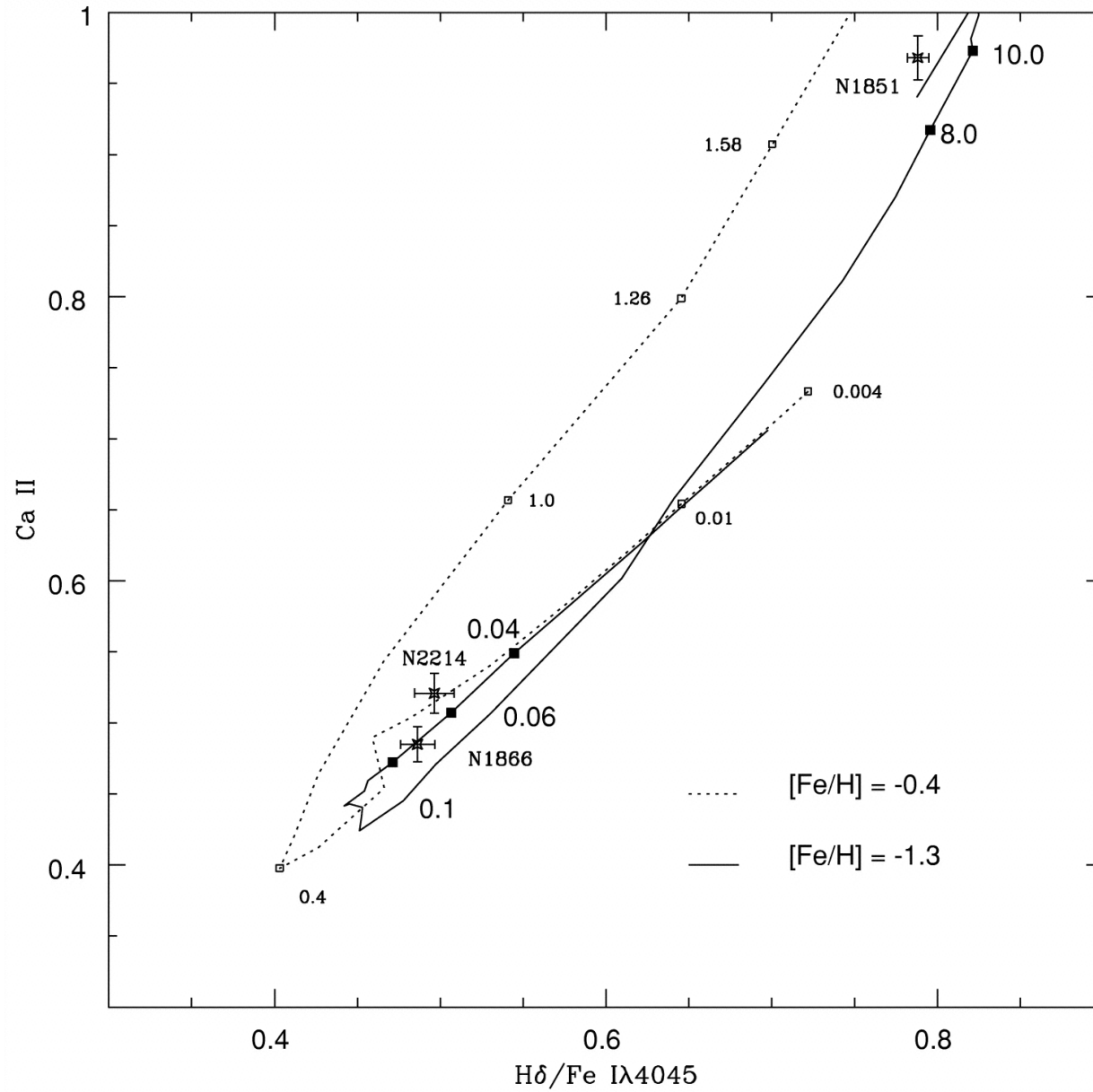
Fig. 12. from Analyzing Starbursts Using Magellanic Cloud Star Clusters as Simple Stellar Populations Leonardi & Rose 2003 AJ 126 1811 doi:10.1086/377617 https://dx.doi.org/10.1086/377617 © 2003. The American Astronomical Society. All rights reserved. Printed in U.S.A.
