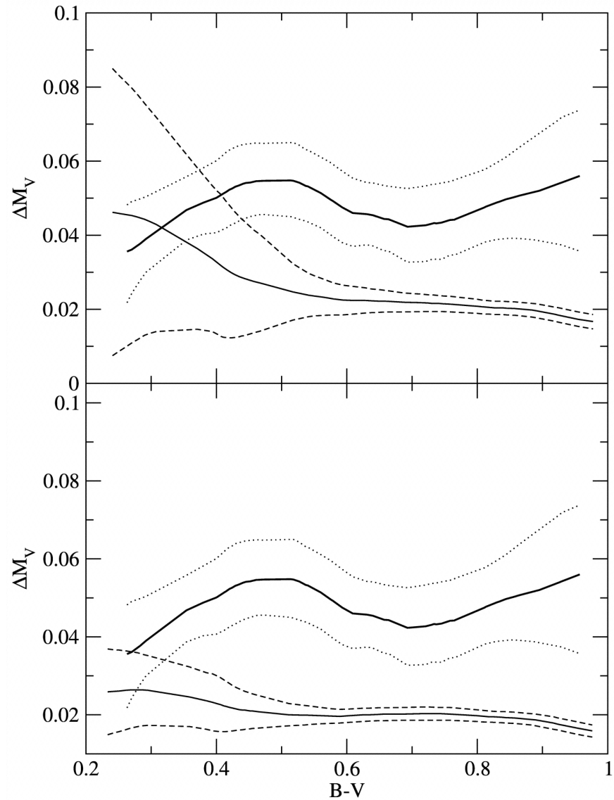
Fig. 3. from The Impact of Pollution on Stellar Evolution Models Dotter & Chaboyer 2003 ApJ 596 496 doi:10.1086/377603 https://dx.doi.org/10.1086/377603 © 2003. The American Astronomical Society. All rights reserved. Printed in U.S.A.
