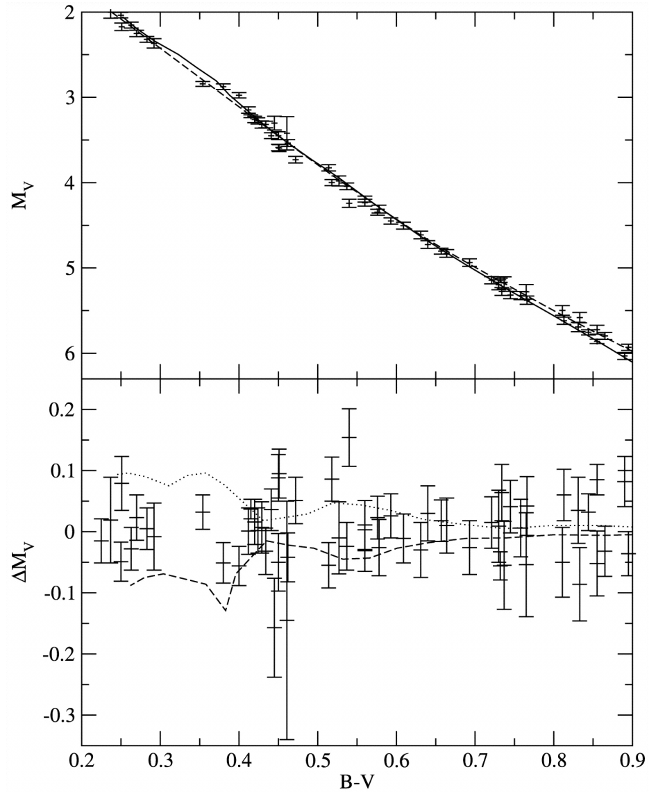
Fig. 2. from The Impact of Pollution on Stellar Evolution Models Dotter & Chaboyer 2003 ApJ 596 496 doi:10.1086/377603 https://dx.doi.org/10.1086/377603 © 2003. The American Astronomical Society. All rights reserved. Printed in U.S.A.
