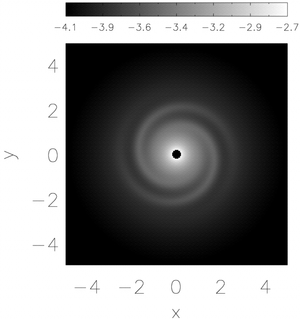
Fig. 7. from Branch, Spur, and Feather Formation in Spiral Galaxies Chakrabarti, Laughlin, & Shu 2003 ApJ 596 220 doi:10.1086/377578 https://dx.doi.org/10.1086/377578 © 2003. The American Astronomical Society. All rights reserved. Printed in U.S.A.
