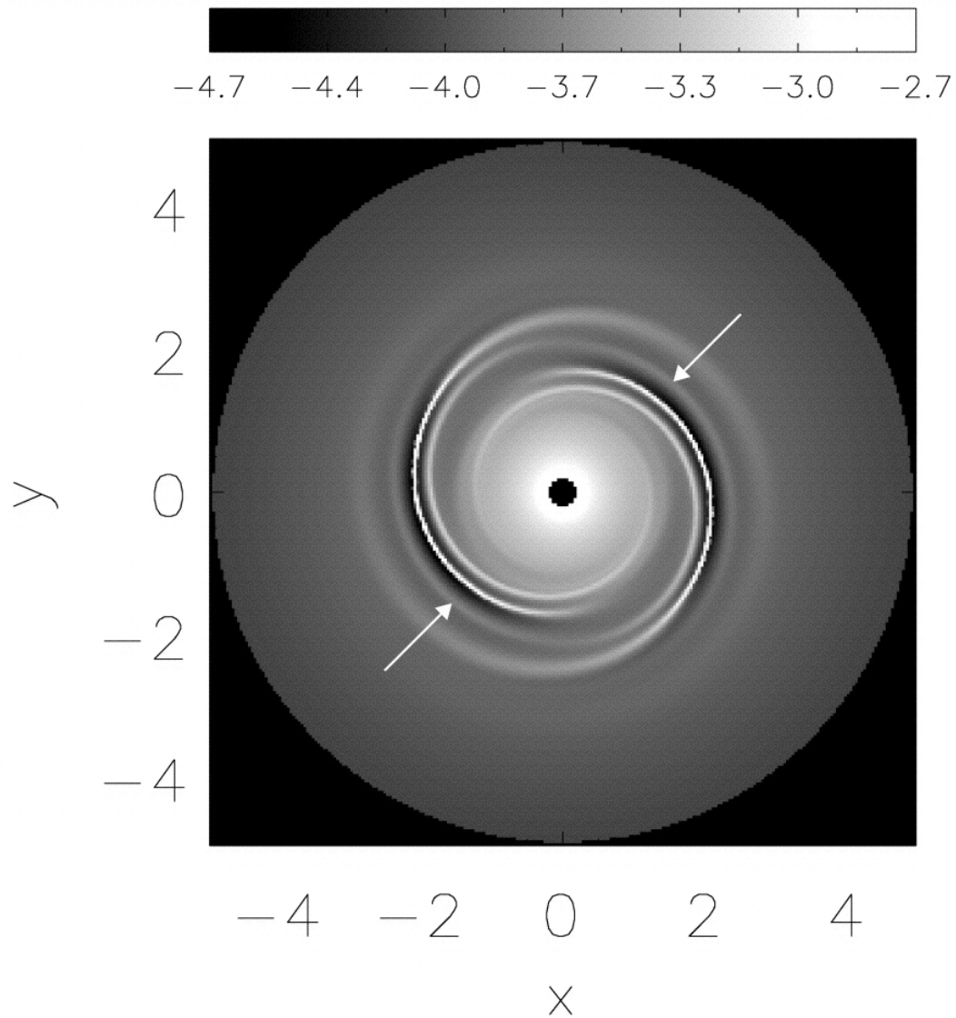
Fig. 5. from Branch, Spur, and Feather Formation in Spiral Galaxies Chakrabarti, Laughlin, & Shu 2003 ApJ 596 220 doi:10.1086/377578 https://dx.doi.org/10.1086/377578 © 2003. The American Astronomical Society. All rights reserved. Printed in U.S.A.
