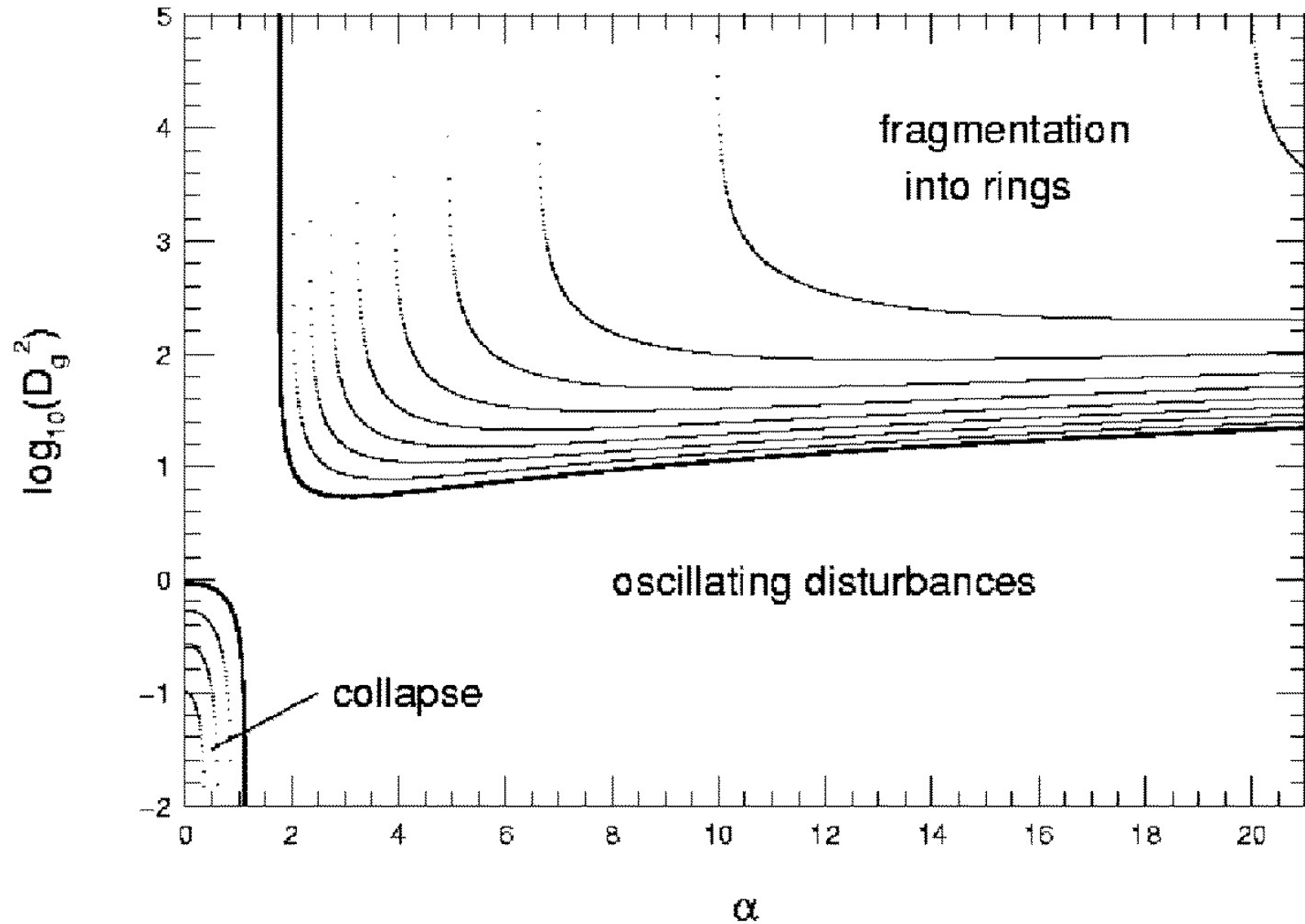
Fig. 2. from Branch, Spur, and Feather Formation in Spiral Galaxies Chakrabarti, Laughlin, & Shu 2003 ApJ 596 220 doi:10.1086/377578 https://dx.doi.org/10.1086/377578 © 2003. The American Astronomical Society. All rights reserved. Printed in U.S.A.
