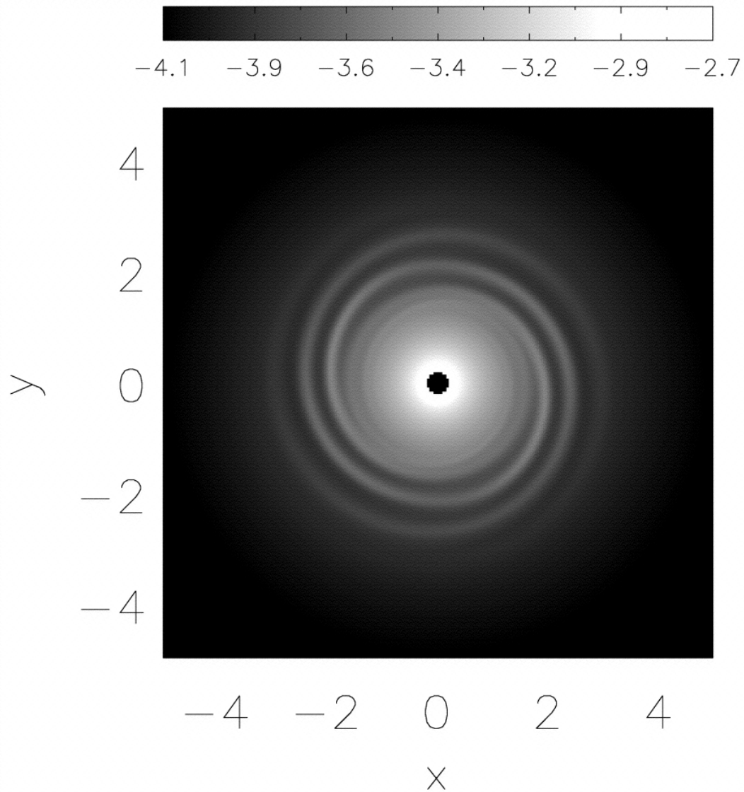
Fig. 12. from Branch, Spur, and Feather Formation in Spiral Galaxies Chakrabarti, Laughlin, & Shu 2003 ApJ 596 220 doi:10.1086/377578 https://dx.doi.org/10.1086/377578 © 2003. The American Astronomical Society. All rights reserved. Printed in U.S.A.
