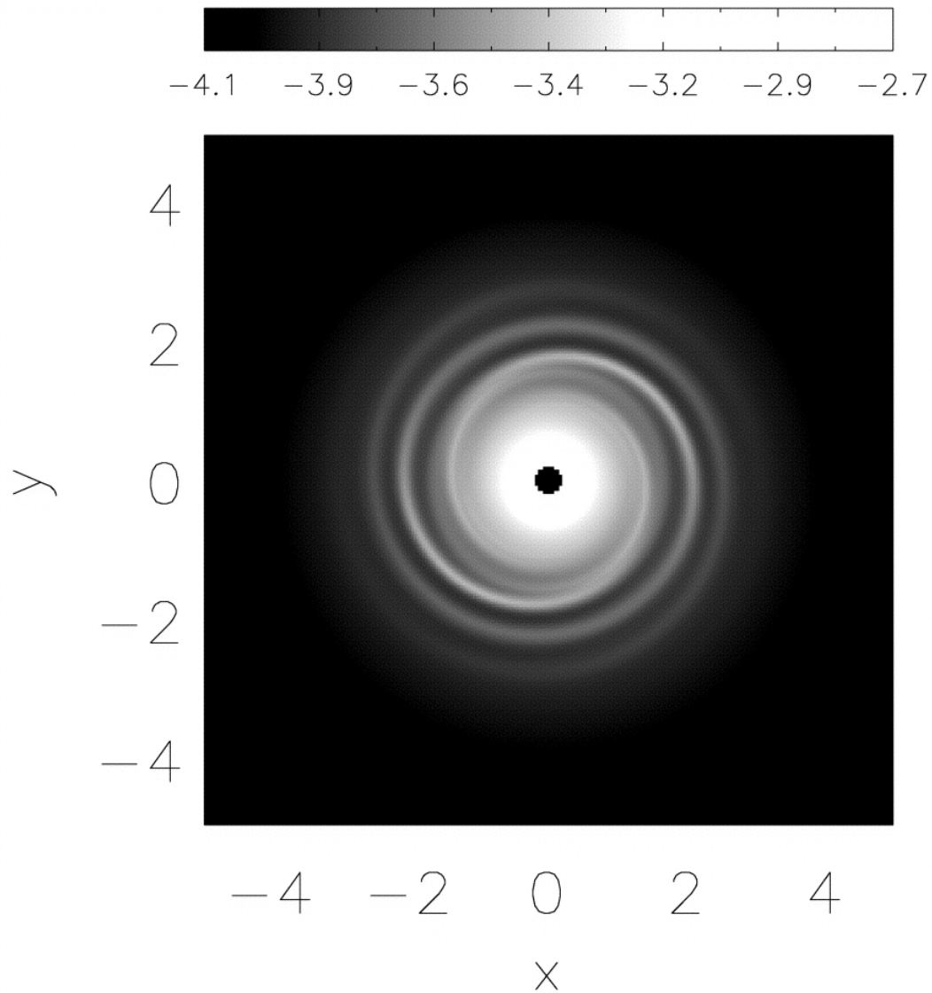
Fig. 11. from Branch, Spur, and Feather Formation in Spiral Galaxies Chakrabarti, Laughlin, & Shu 2003 ApJ 596 220 doi:10.1086/377578 https://dx.doi.org/10.1086/377578 © 2003. The American Astronomical Society. All rights reserved. Printed in U.S.A.
