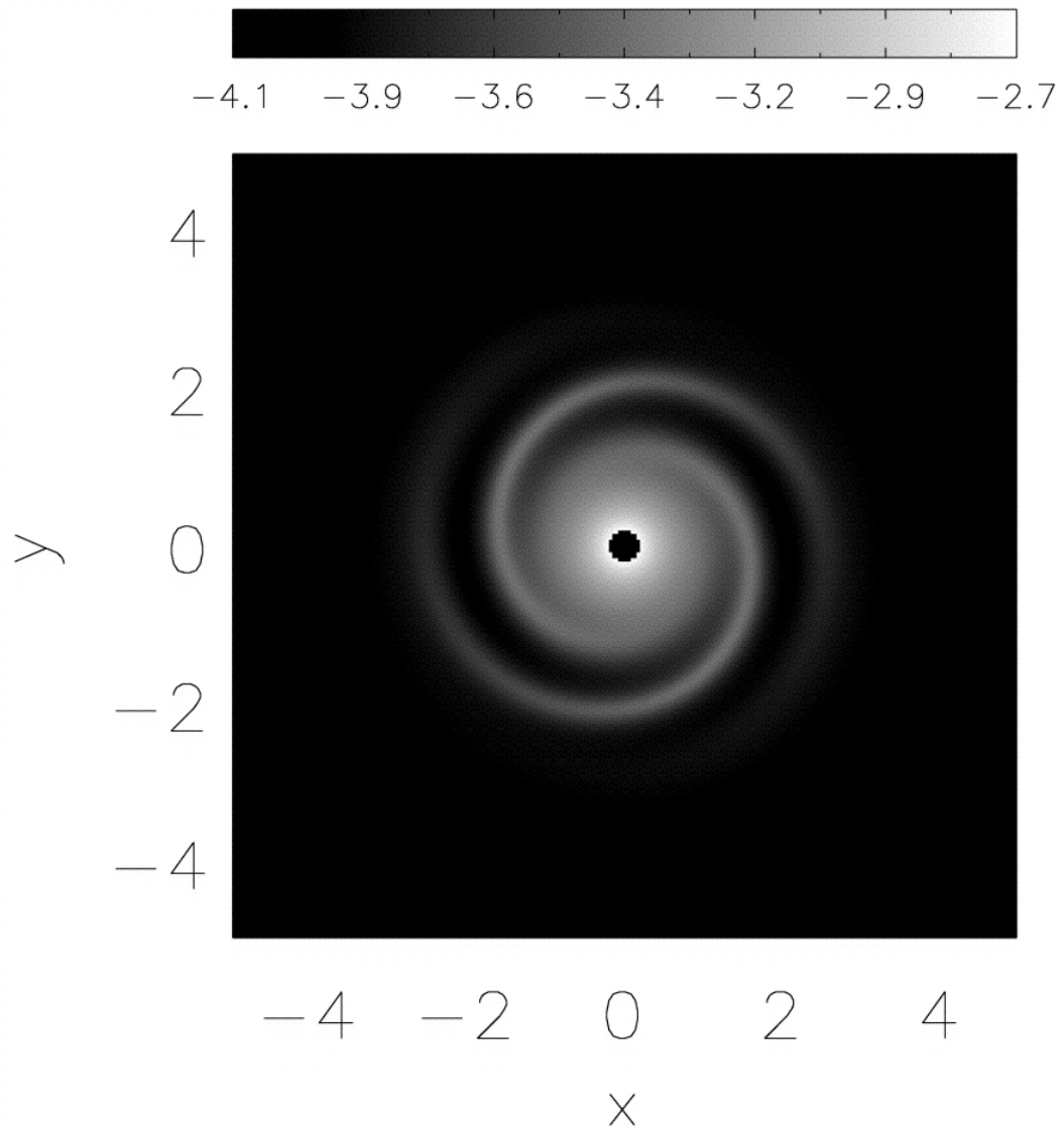
Fig. 10. from Branch, Spur, and Feather Formation in Spiral Galaxies Chakrabarti, Laughlin, & Shu 2003 ApJ 596 220 doi:10.1086/377578 https://dx.doi.org/10.1086/377578 © 2003. The American Astronomical Society. All rights reserved. Printed in U.S.A.
