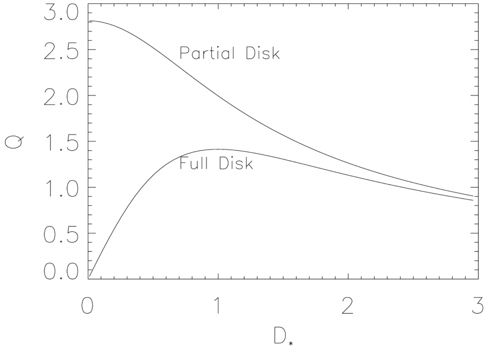
Fig. 1. from Branch, Spur, and Feather Formation in Spiral Galaxies Chakrabarti, Laughlin, & Shu 2003 ApJ 596 220 doi:10.1086/377578 https://dx.doi.org/10.1086/377578 © 2003. The American Astronomical Society. All rights reserved. Printed in U.S.A.
