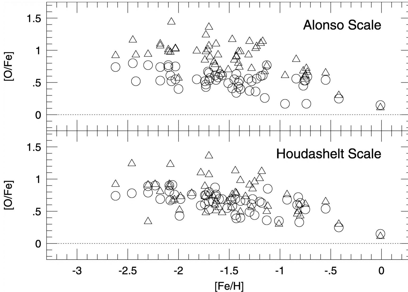
Fig. 9. from Oxygen Abundances in Metalpoor Stars Fulbright & Johnson 2003 ApJ 595 1154 doi:10.1086/377443 https://dx.doi.org/10.1086/377443
