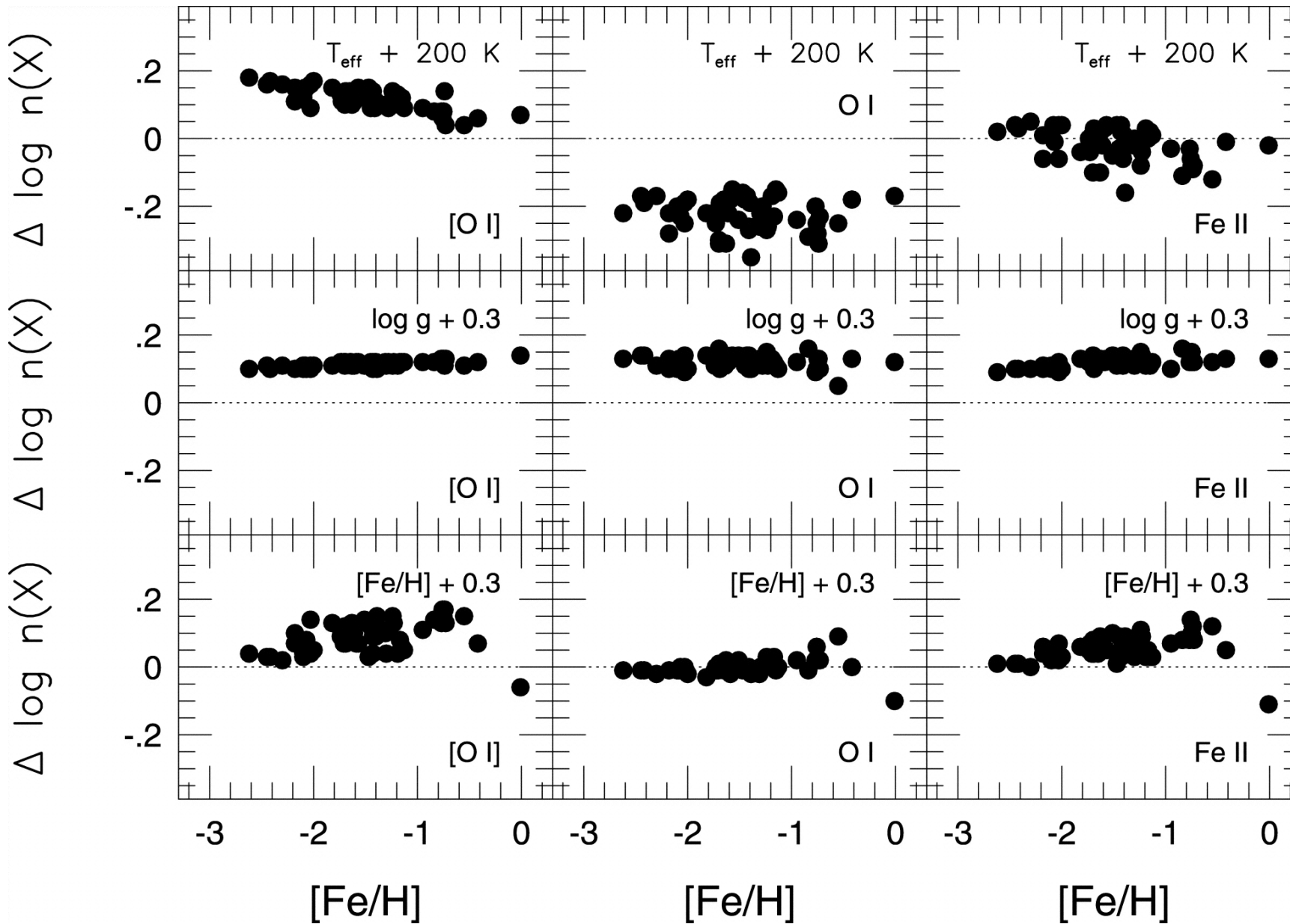
Fig. 8. from Oxygen Abundances in Metalpoor Stars Fulbright & Johnson 2003 ApJ 595 1154 doi:10.1086/377443 https://dx.doi.org/10.1086/377443
