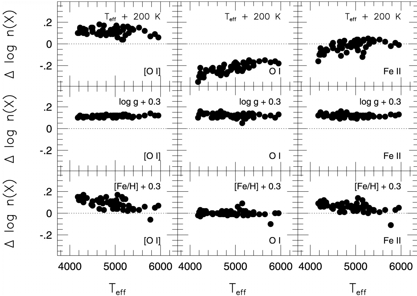
Fig. 6. from Oxygen Abundances in Metalpoor Stars Fulbright & Johnson 2003 ApJ 595 1154 doi:10.1086/377443 https://dx.doi.org/10.1086/377443
