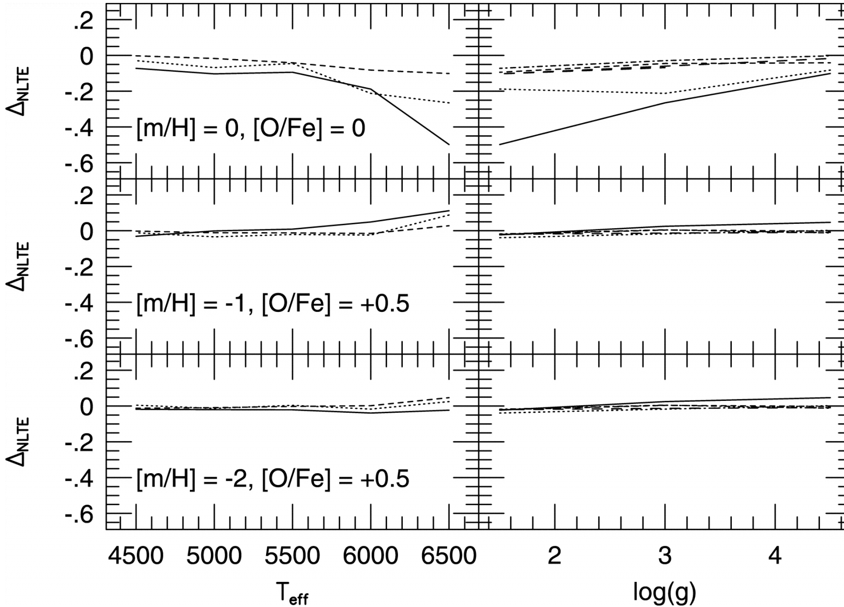
Fig. 4. from Oxygen Abundances in Metalpoor Stars Fulbright & Johnson 2003 ApJ 595 1154 doi:10.1086/377443 https://dx.doi.org/10.1086/377443
