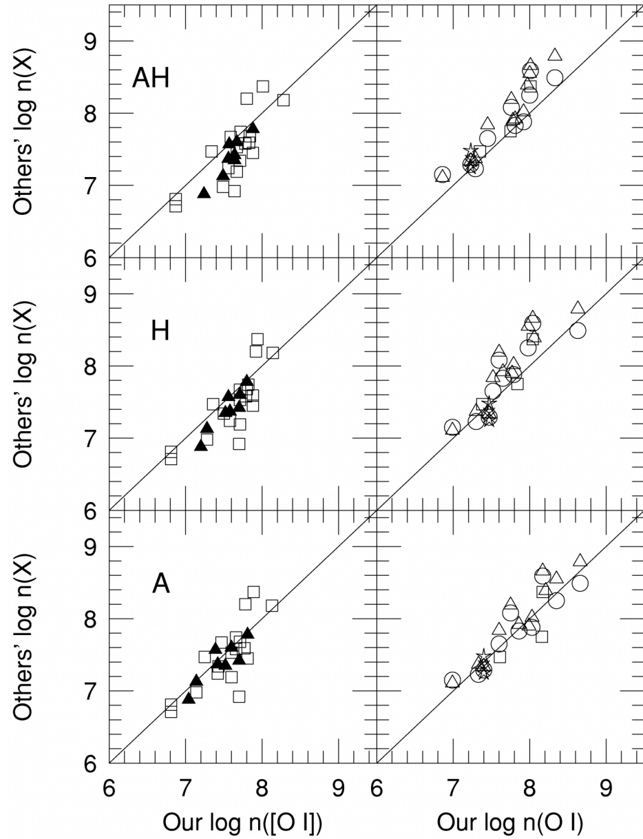
Fig. 14. from Oxygen Abundances in Metalpoor Stars Fulbright & Johnson 2003 ApJ 595 1154 doi:10.1086/377443 https://dx.doi.org/10.1086/377443 © 2003. The American Astronomical Society. All rights reserved. Printed in U.S.A.
