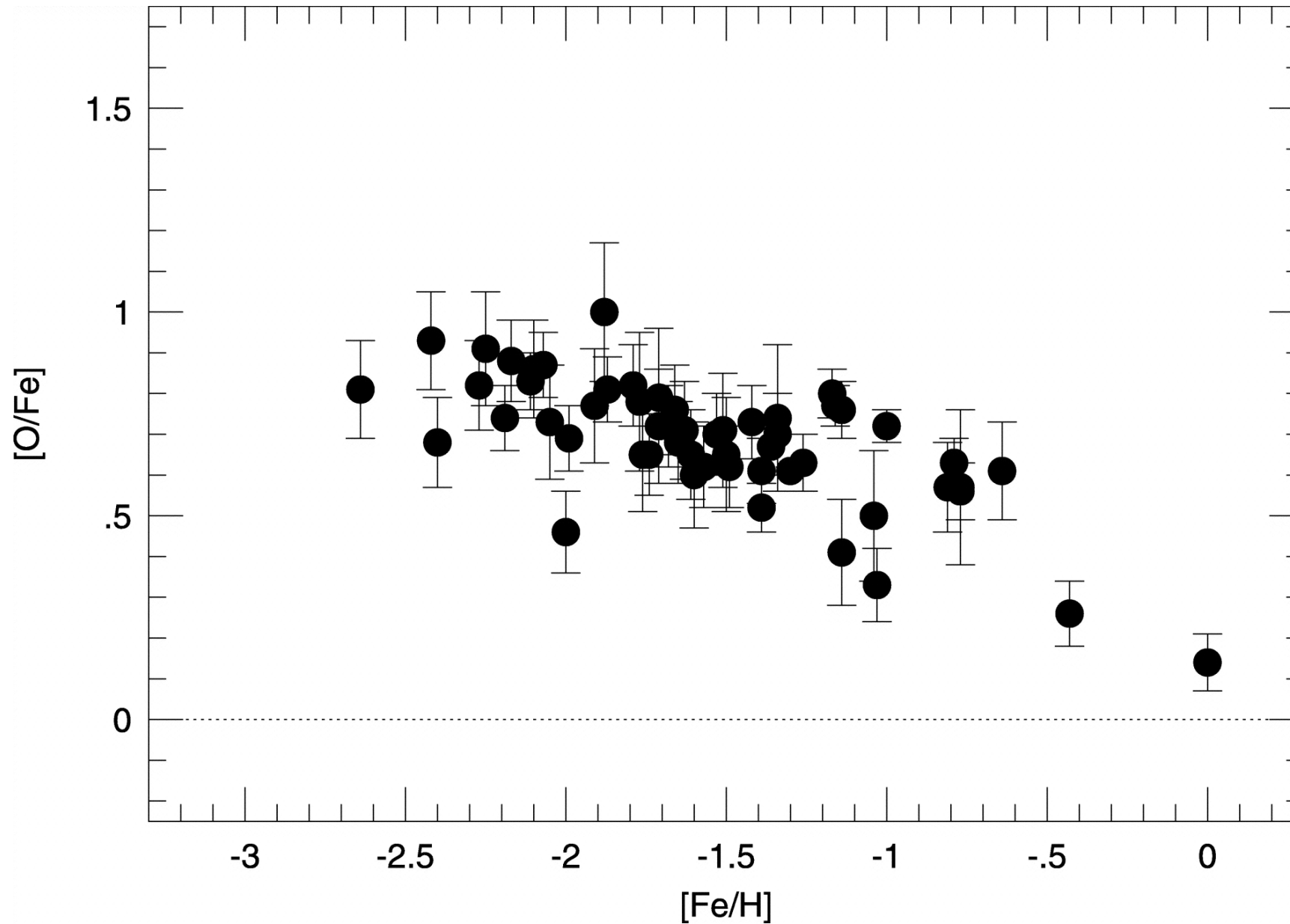
Fig. 13. from Oxygen Abundances in Metalpoor Stars Fulbright & Johnson 2003 ApJ 595 1154 doi:10.1086/377443 https://dx.doi.org/10.1086/377443
