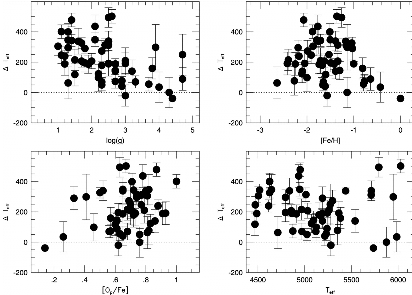
Fig. 12. from Oxygen Abundances in Metalpoor Stars Fulbright & Johnson 2003 ApJ 595 1154 doi:10.1086/377443 https://dx.doi.org/10.1086/377443
