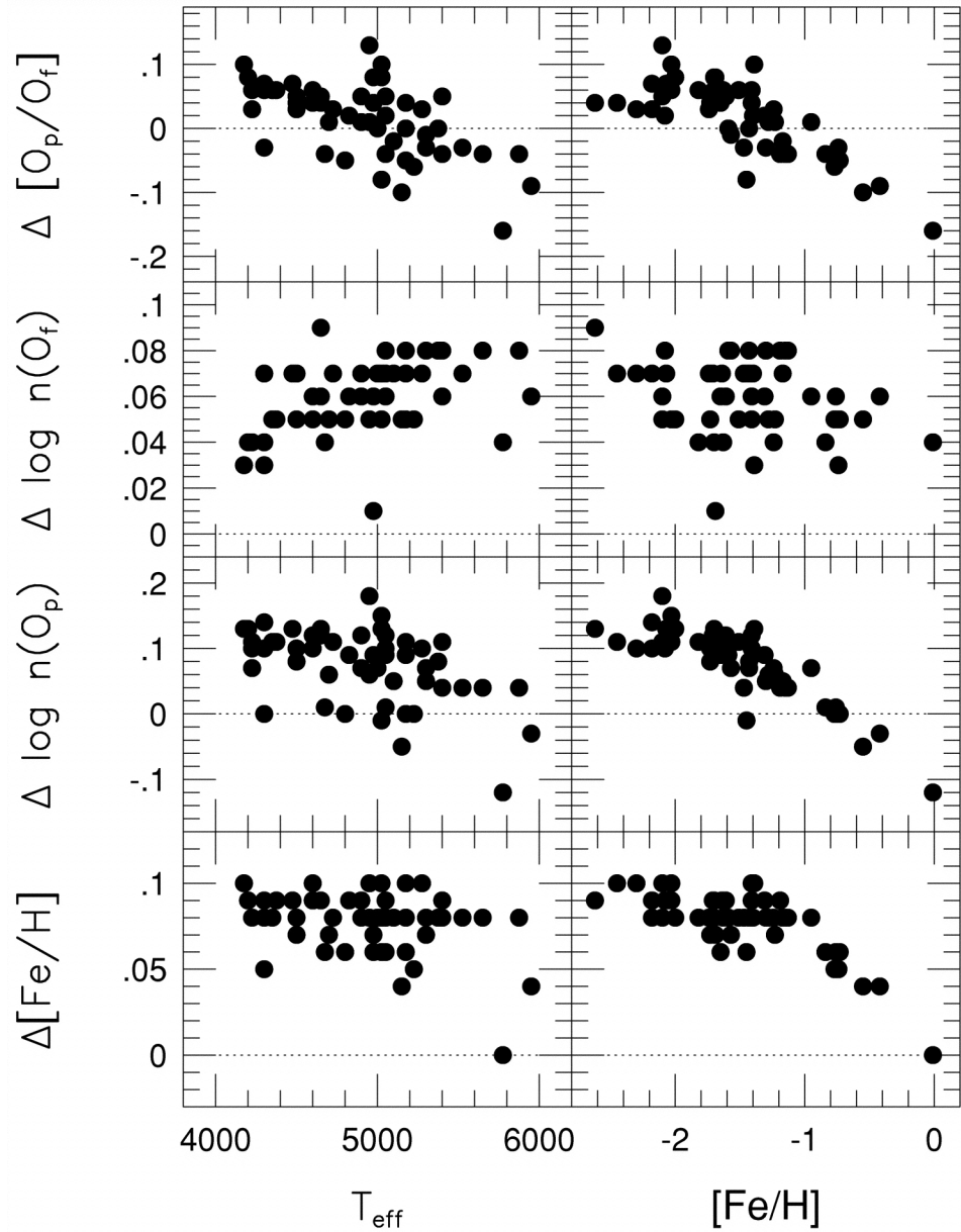
Fig. 11. from Oxygen Abundances in Metalpoor Stars Fulbright & Johnson 2003 ApJ 595 1154 doi:10.1086/377443 https://dx.doi.org/10.1086/377443 © 2003. The American Astronomical Society. All rights reserved. Printed in U.S.A.
