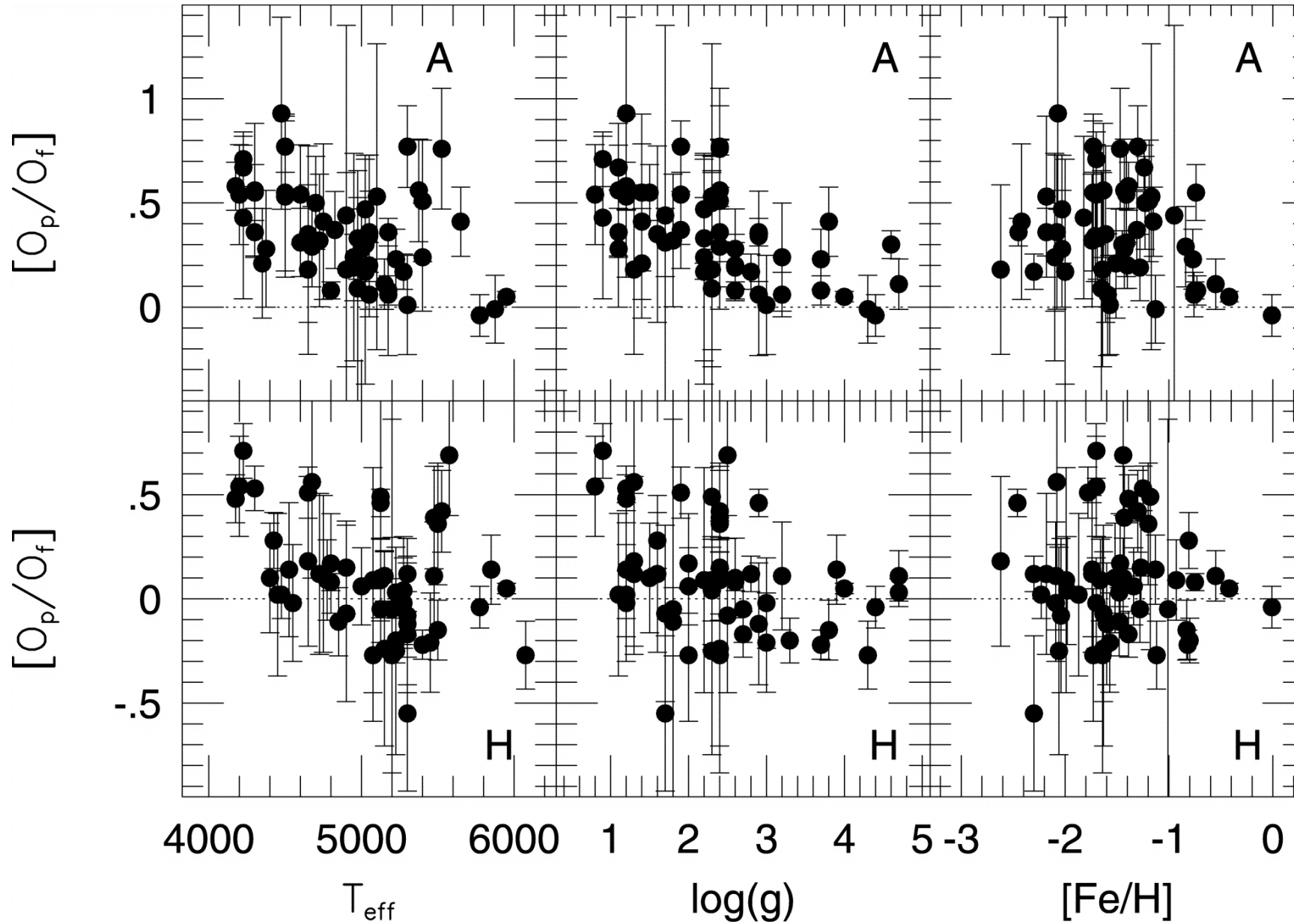
Fig. 10. from Oxygen Abundances in Metalpoor Stars Fulbright & Johnson 2003 ApJ 595 1154 doi:10.1086/377443 https://dx.doi.org/10.1086/377443
