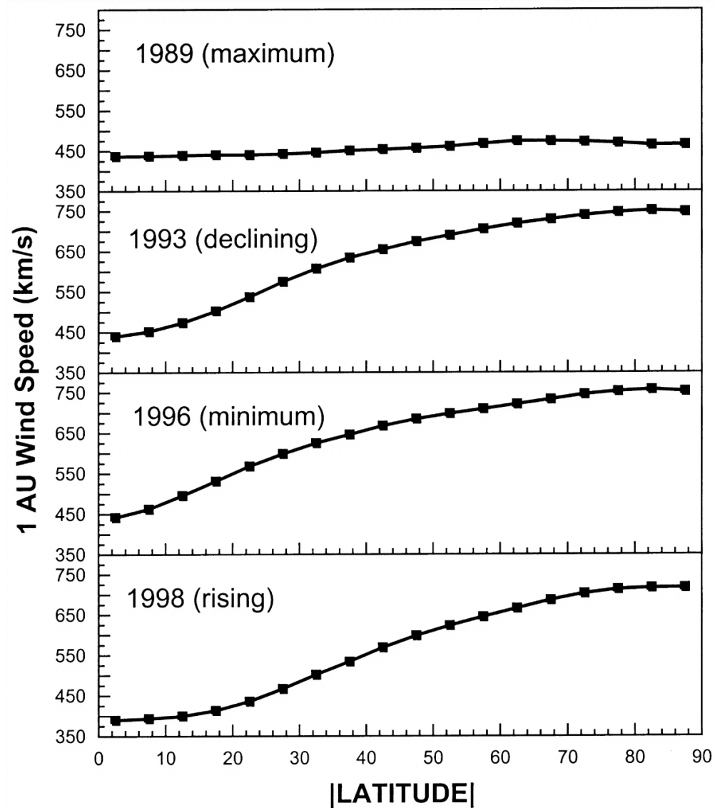
Fig. 5. from Solar Wind Speed and Temperature Outside 10 AU and the Termination Shock Whang et al. 2003 ApJ 589 635 doi:10.1086/374595 https://dx.doi.org/10.1086/374595 © 2003. The American Astronomical Society. All rights reserved. Printed in U.S.A.
