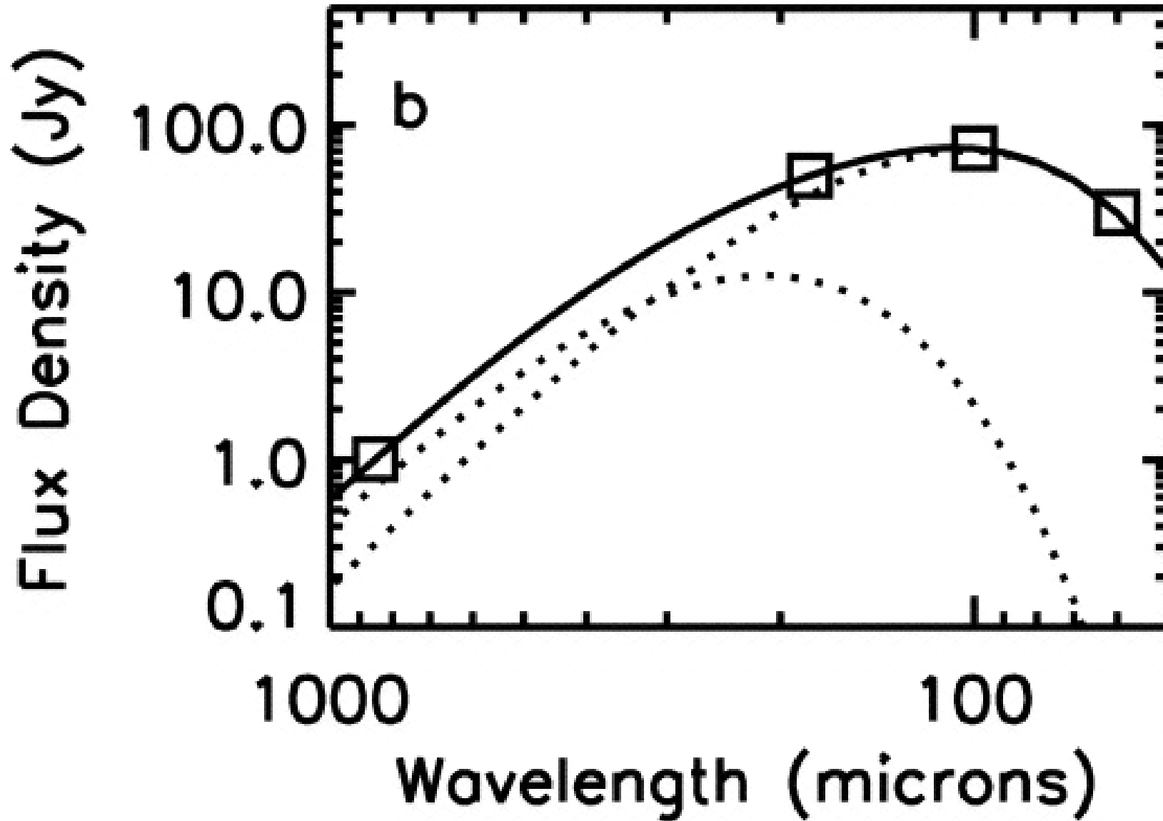
Fig. 5. from Dust Temperatures in the Infrared Space Observatory Atlas of Bright Spiral Galaxies Bendo et al. 2003 AJ 125 2361 doi:10.1086/374361 https://dx.doi.org/10.1086/374361 © 2003. The American Astronomical Society. All rights reserved. Printed in U.S.A.
