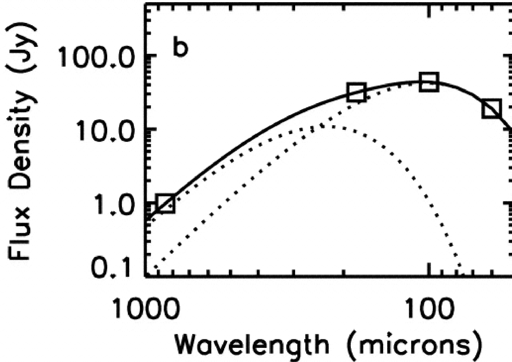
Fig. 3. from Dust Temperatures in the Infrared Space Observatory Atlas of Bright Spiral Galaxies Bendo et al. 2003 AJ 125 2361 doi:10.1086/374361 https://dx.doi.org/10.1086/374361 © 2003. The American Astronomical Society. All rights reserved. Printed in U.S.A.
