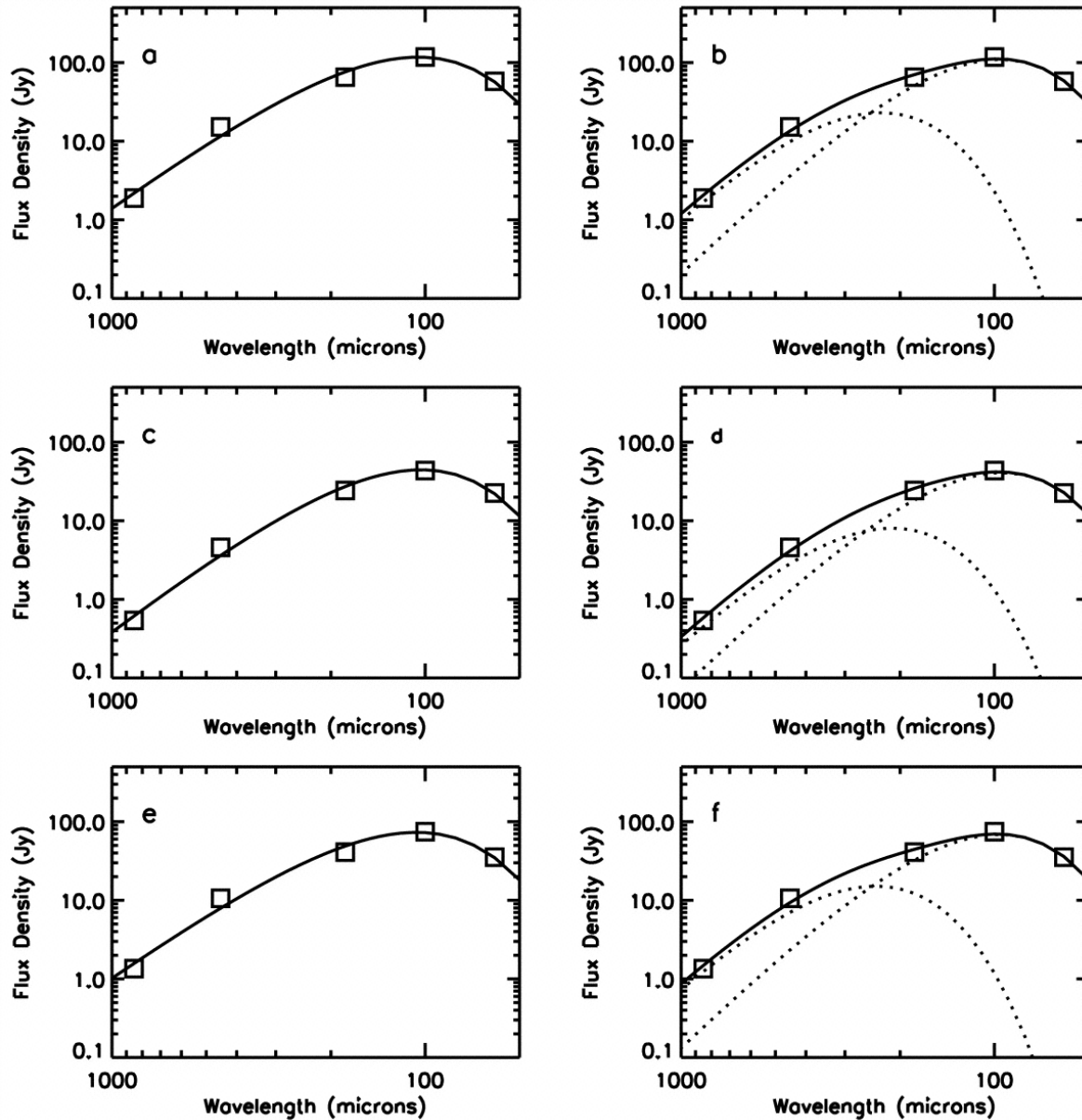
Fig. 2. from Dust Temperatures in the Infrared Space Observatory Atlas of Bright Spiral Galaxies Bendo et al. 2003 AJ 125 2361 doi:10.1086/374361 https://dx.doi.org/10.1086/374361 © 2003. The American Astronomical Society. All rights reserved. Printed in U.S.A.
