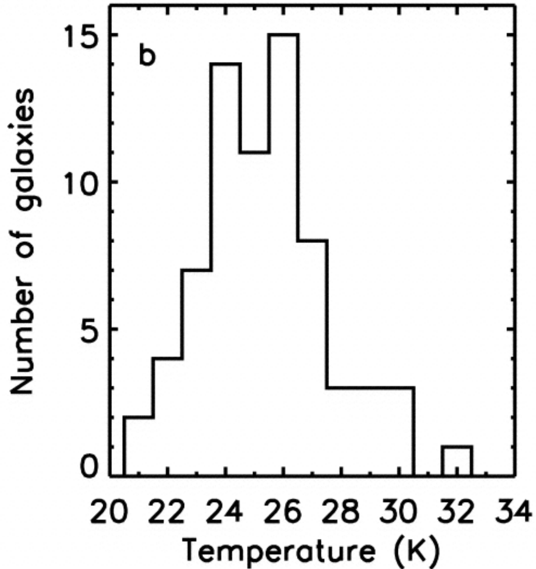
Fig. 1. from Dust Temperatures in the Infrared Space Observatory Atlas of Bright Spiral Galaxies Bendo et al. 2003 AJ 125 2361 doi:10.1086/374361 https://dx.doi.org/10.1086/374361 © 2003. The American Astronomical Society. All rights reserved. Printed in U.S.A.
