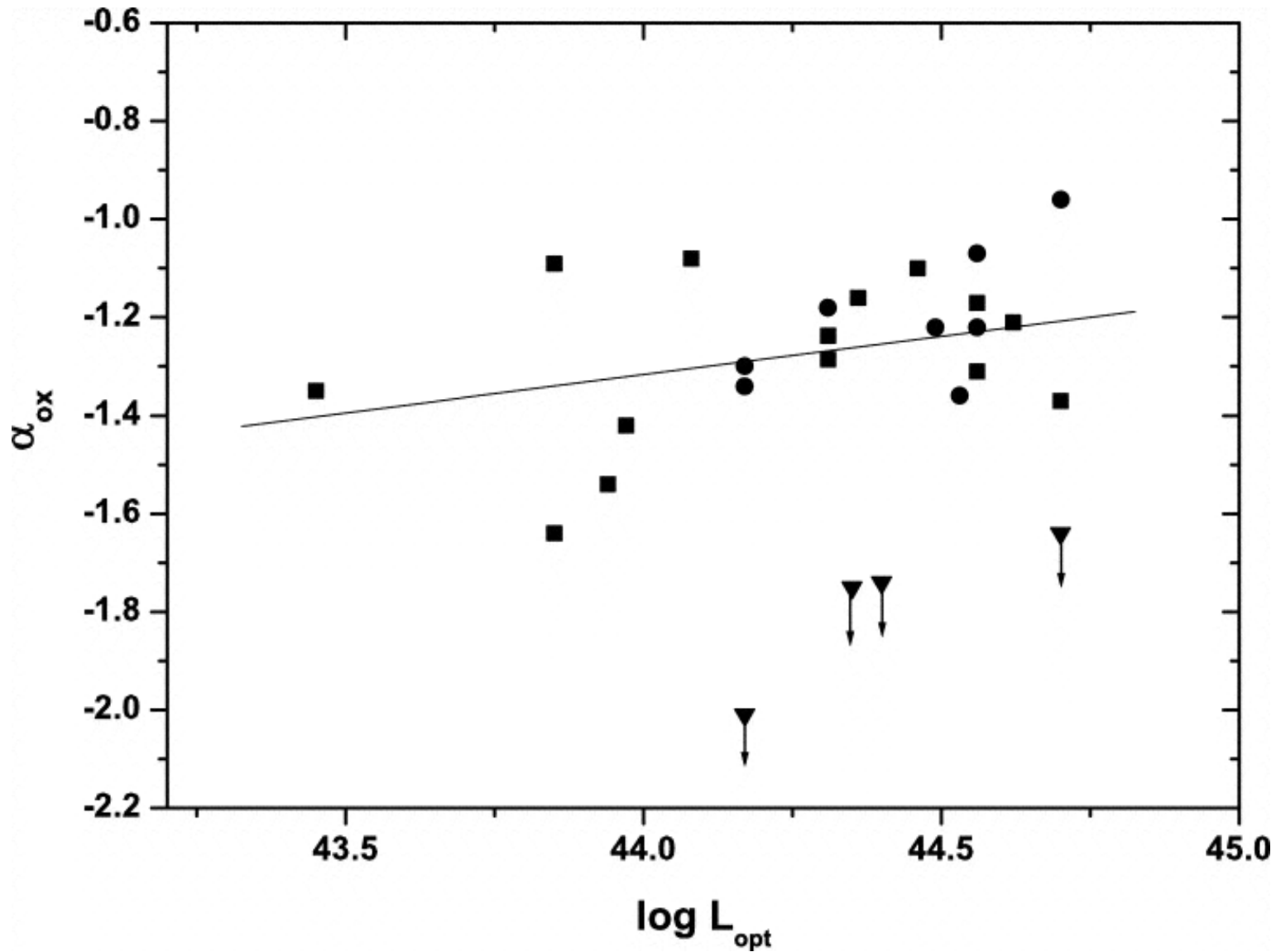
Fig. 8. from A Multiwavelength Study of NarrowLine Seyfert 1 Galaxies from the Second Byurakan Survey Stepanian et al. 2003 ApJ 588 746 doi:10.1086/374215 https://dx.doi.org/10.1086/374215 © 2003. The American Astronomical Society. All rights reserved. Printed in U.S.A.
