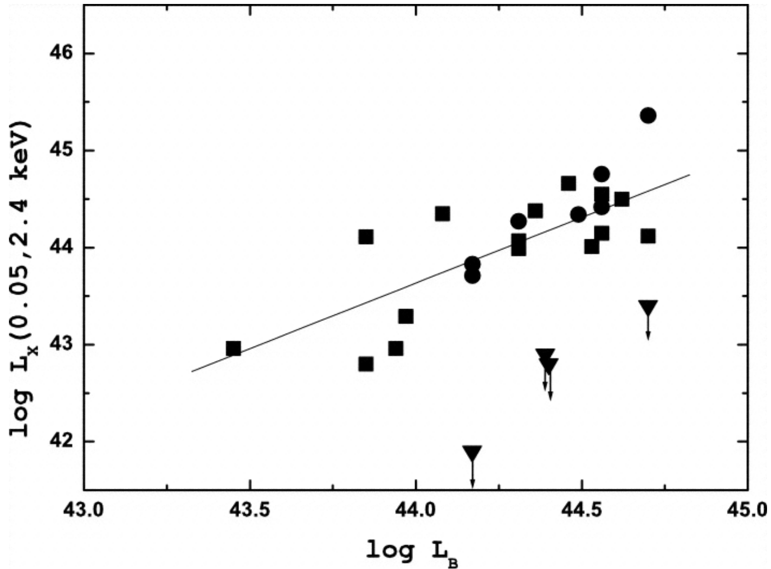
Fig. 4. from A Multiwavelength Study of NarrowLine Seyfert 1 Galaxies from the Second Byurakan Survey Stepanian et al. 2003 ApJ 588 746 doi:10.1086/374215 https://dx.doi.org/10.1086/374215 © 2003. The American Astronomical Society. All rights reserved. Printed in U.S.A.
