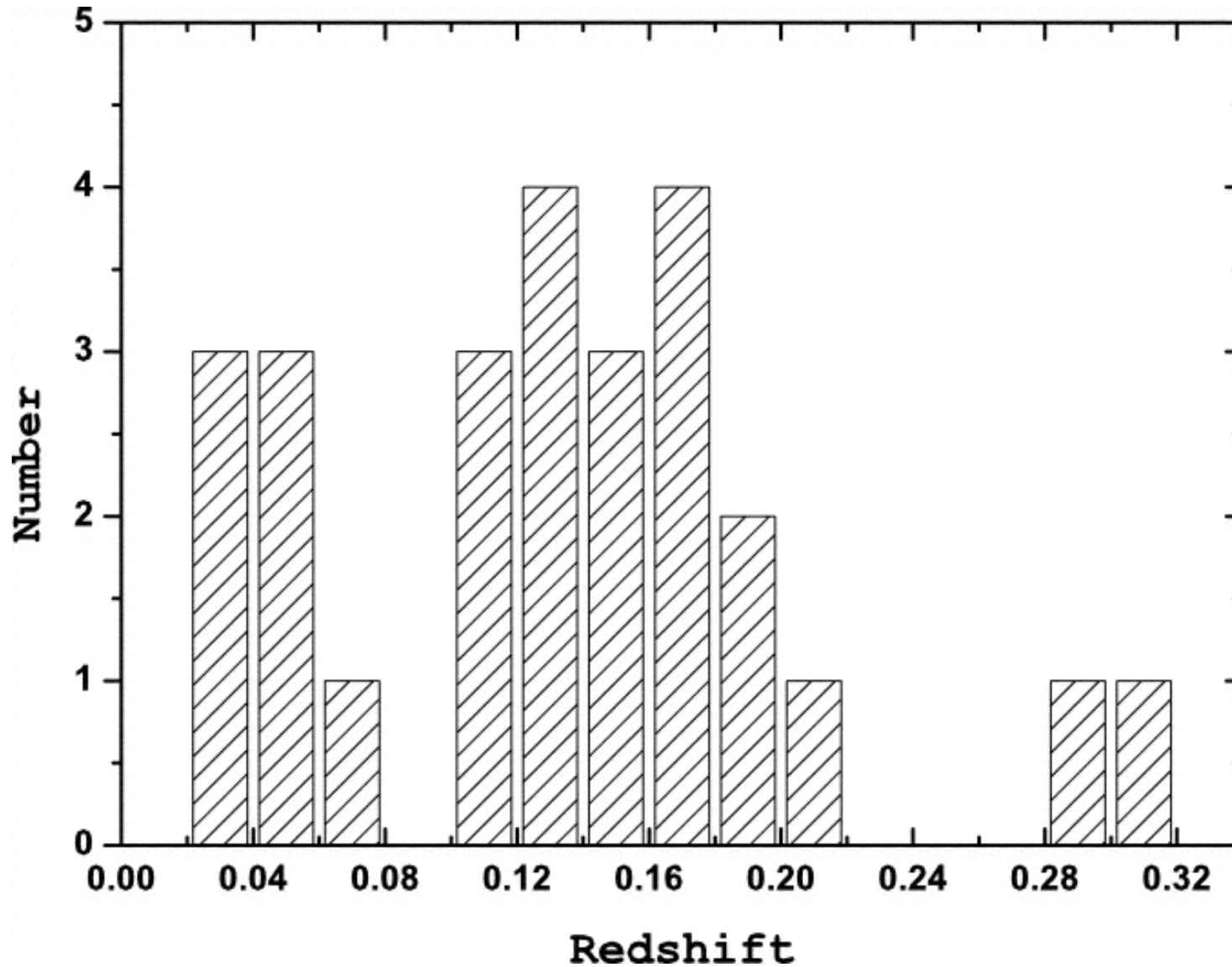
Fig. 1. from A Multiwavelength Study of NarrowLine Seyfert 1 Galaxies from the Second Byurakan Survey Stepanian et al. 2003 ApJ 588 746 doi:10.1086/374215 https://dx.doi.org/10.1086/374215 © 2003. The American Astronomical Society. All rights reserved. Printed in U.S.A.
