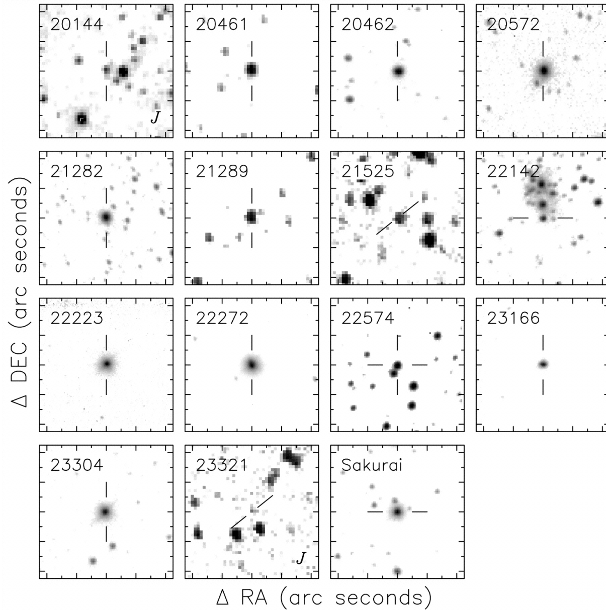
Fig. 1. from NearInfrared Photometric Survey of Proto-Planetary Nebula Candidates Ueta et al. 2003 AJ 125 2227 doi:10.1086/373928 https://dx.doi.org/10.1086/373928 © 2003. The American Astronomical Society. All rights reserved. Printed in U.S.A.
