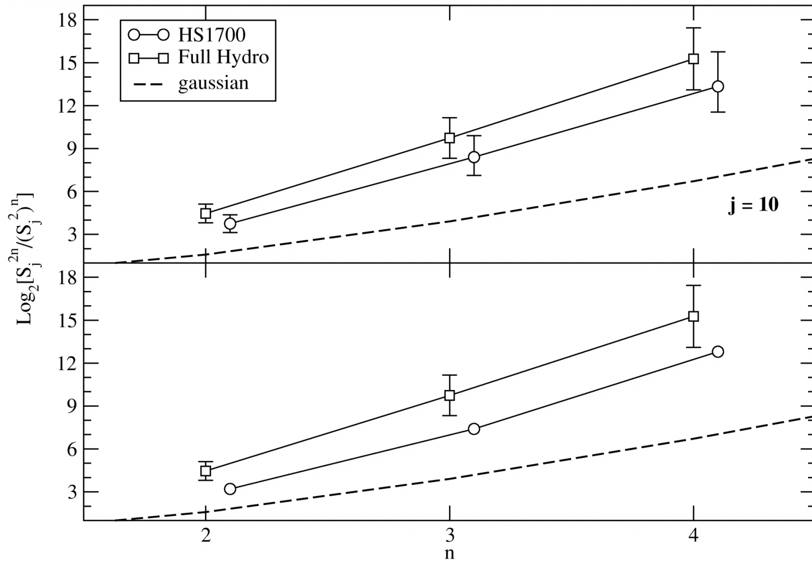
Fig. 13. from Intermittent Features of the Quasar Ly Transmitted Flux: Results from Cosmological Hydrodynamic Simulations Feng, Pando, & Fang 2003 ApJ 587 487 doi:10.1086/368306 https://dx.doi.org/10.1086/368306 © 2003. The American Astronomical Society. All rights reserved. Printed in U.S.A.
