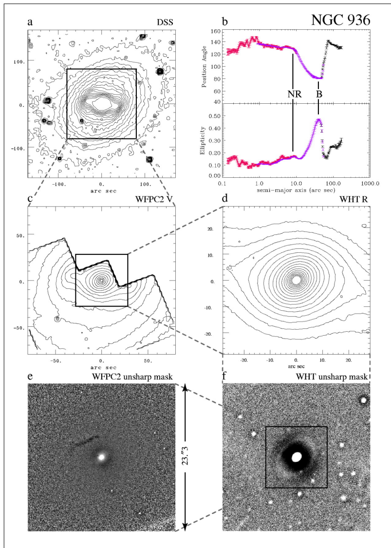
Fig. 8. from An Imaging Survey of EarlyType Barred Galaxies Erwin & Sparke 2003 ApJS 146 299 doi:10.1086/367885 https://dx.doi.org/10.1086/367885 © 2003. The American Astronomical Society. All rights reserved. Printed in U.S.A.
