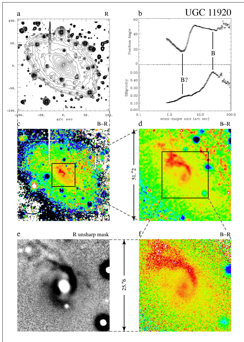
Fig. 40. from An Imaging Survey of EarlyType Barred Galaxies Erwin & Sparke 2003 ApJS 146 299 doi:10.1086/367885 https://dx.doi.org/10.1086/367885 © 2003. The American Astronomical Society. All rights reserved. Printed in U.S.A.
