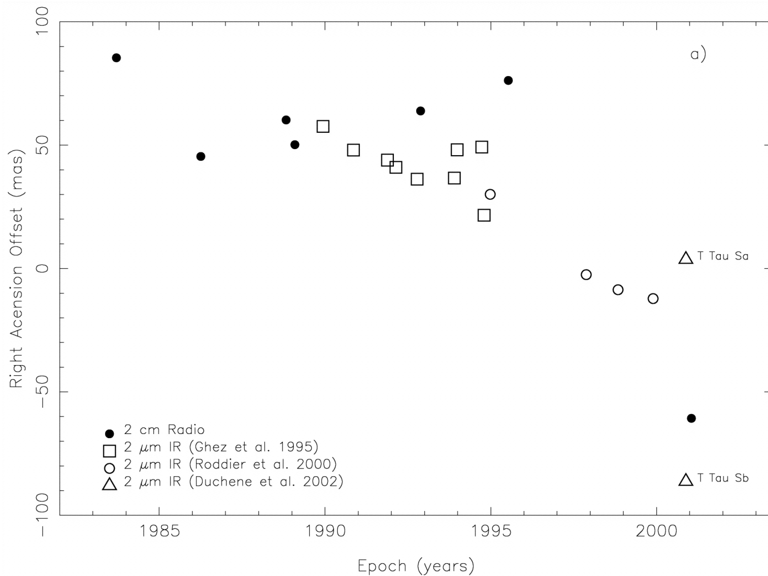
Fig. 5. from The Variable Radio Source T Tauri Johnston et al. 2003 AJ 125 858 doi:10.1086/345727 https://dx.doi.org/10.1086/345727 © 2003. The American Astronomical Society. All rights reserved. Printed in U.S.A.
