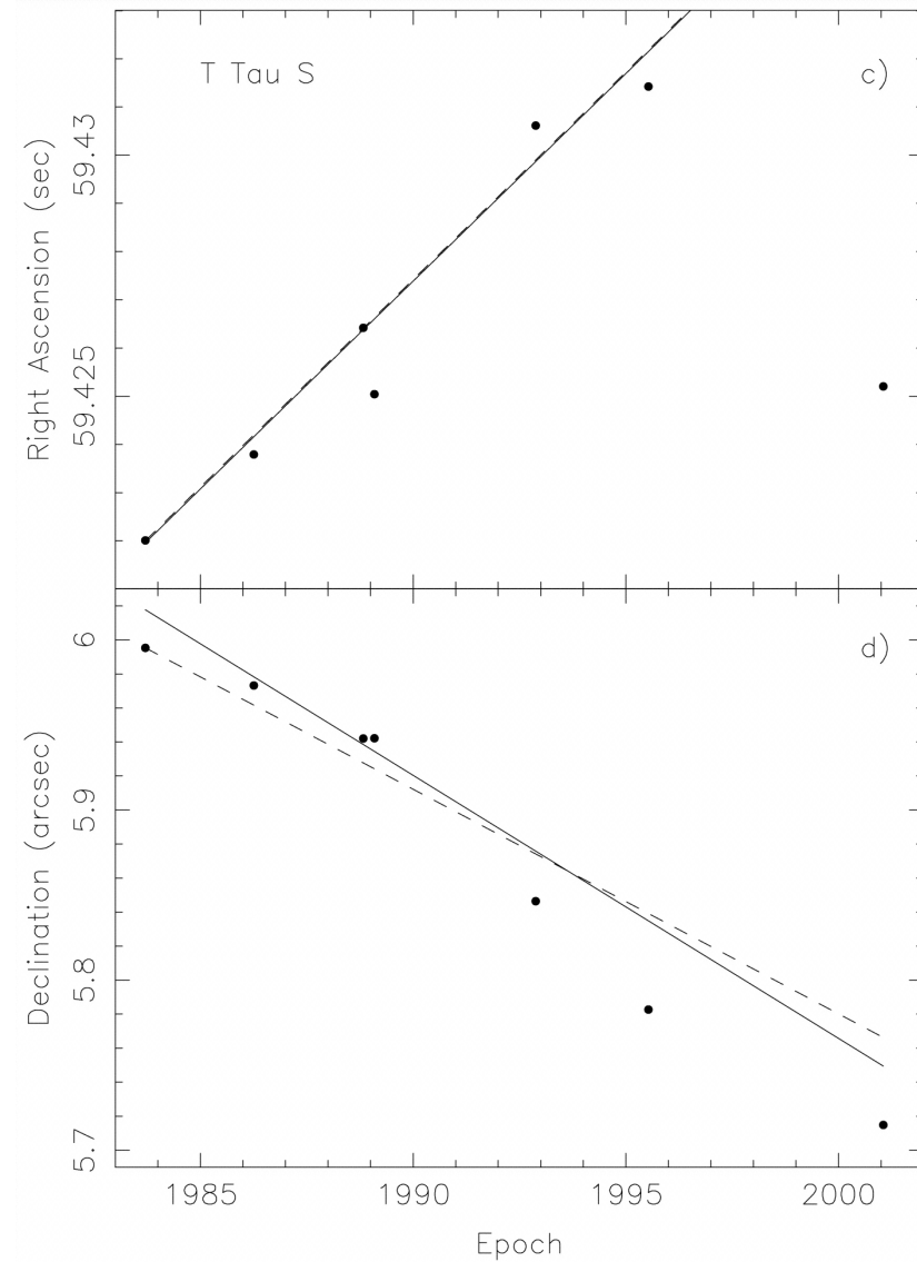
Fig. 4. from The Variable Radio Source T Tauri Johnston et al. 2003 AJ 125 858 doi:10.1086/345727 https://dx.doi.org/10.1086/345727 © 2003. The American Astronomical Society. All rights reserved. Printed in U.S.A.
