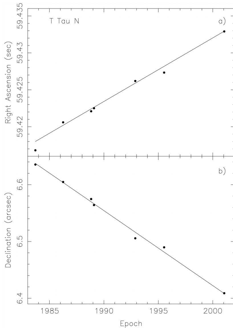
Fig. 4. from The Variable Radio Source T Tauri Johnston et al. 2003 AJ 125 858 doi:10.1086/345727 https://dx.doi.org/10.1086/345727 © 2003. The American Astronomical Society. All rights reserved. Printed in U.S.A.
