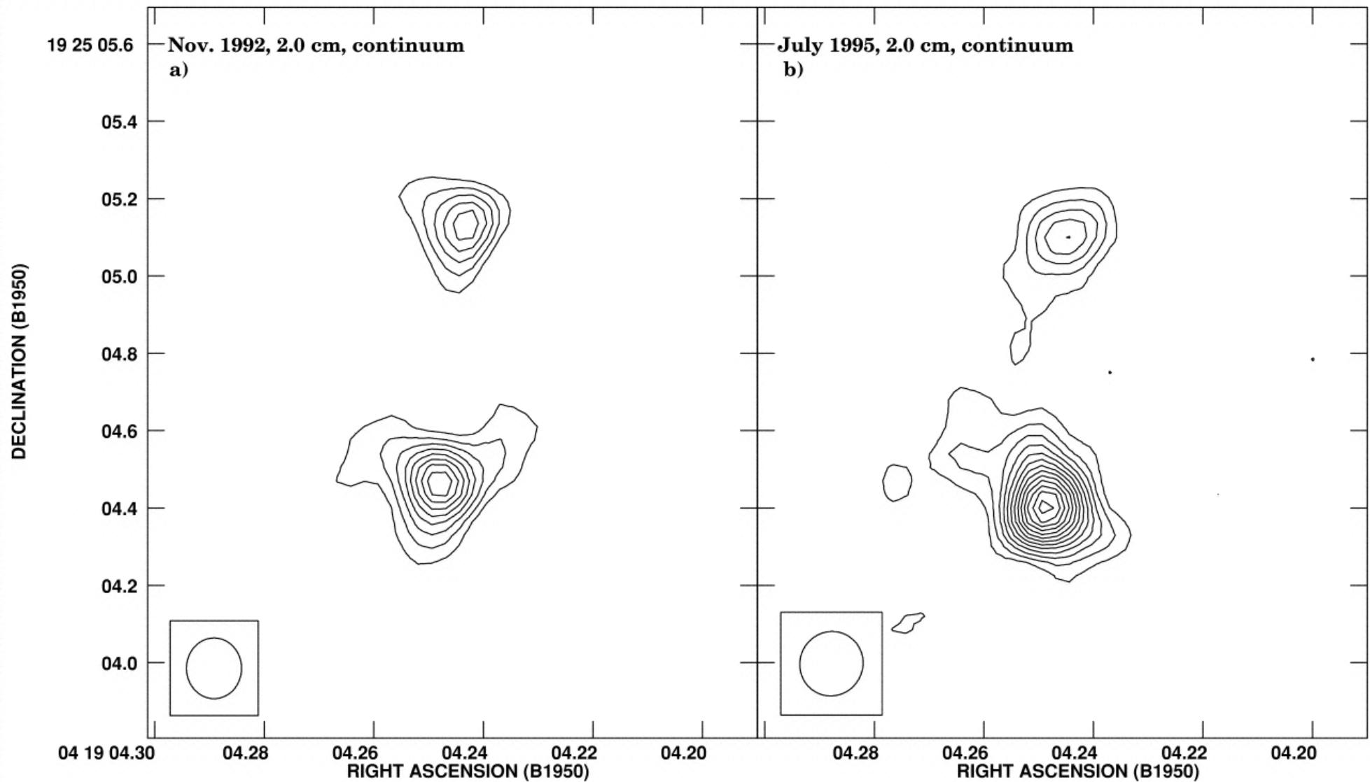
Fig. 2. from The Variable Radio Source T Tauri Johnston et al. 2003 AJ 125 858 doi:10.1086/345727 https://dx.doi.org/10.1086/345727 © 2003. The American Astronomical Society. All rights reserved. Printed in U.S.A.
