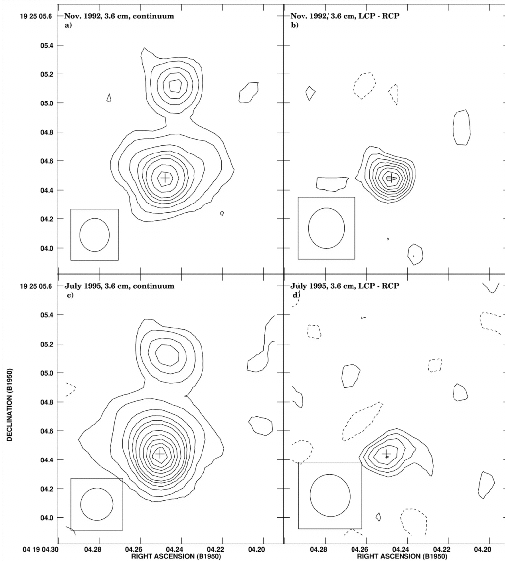
Fig. 1. from The Variable Radio Source T Tauri Johnston et al. 2003 AJ 125 858 doi:10.1086/345727 https://dx.doi.org/10.1086/345727 © 2003. The American Astronomical Society. All rights reserved. Printed in U.S.A.
