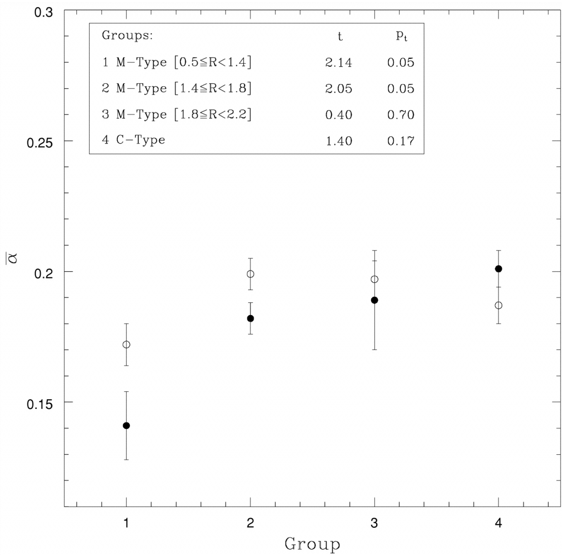
Fig. 4. from On the Origin of Long Secondary Periods in Semiregular Variables Olivier & Wood 2003 ApJ 584 1035 doi:10.1086/345715 https://dx.doi.org/10.1086/345715 © 2003. The American Astronomical Society. All rights reserved. Printed in U.S.A.
