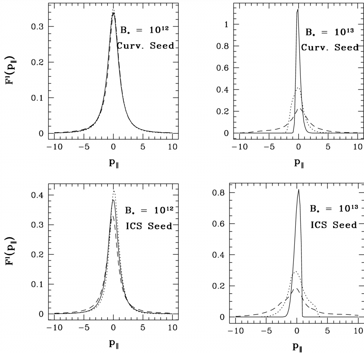
Fig. 9. from Pair Creation in the Pulsar Magnetosphere Arendt & Eilek 2002 ApJ 581 451 doi:10.1086/344133 https://dx.doi.org/10.1086/344133 © 2002. The American Astronomical Society. All rights reserved. Printed in U.S.A.
