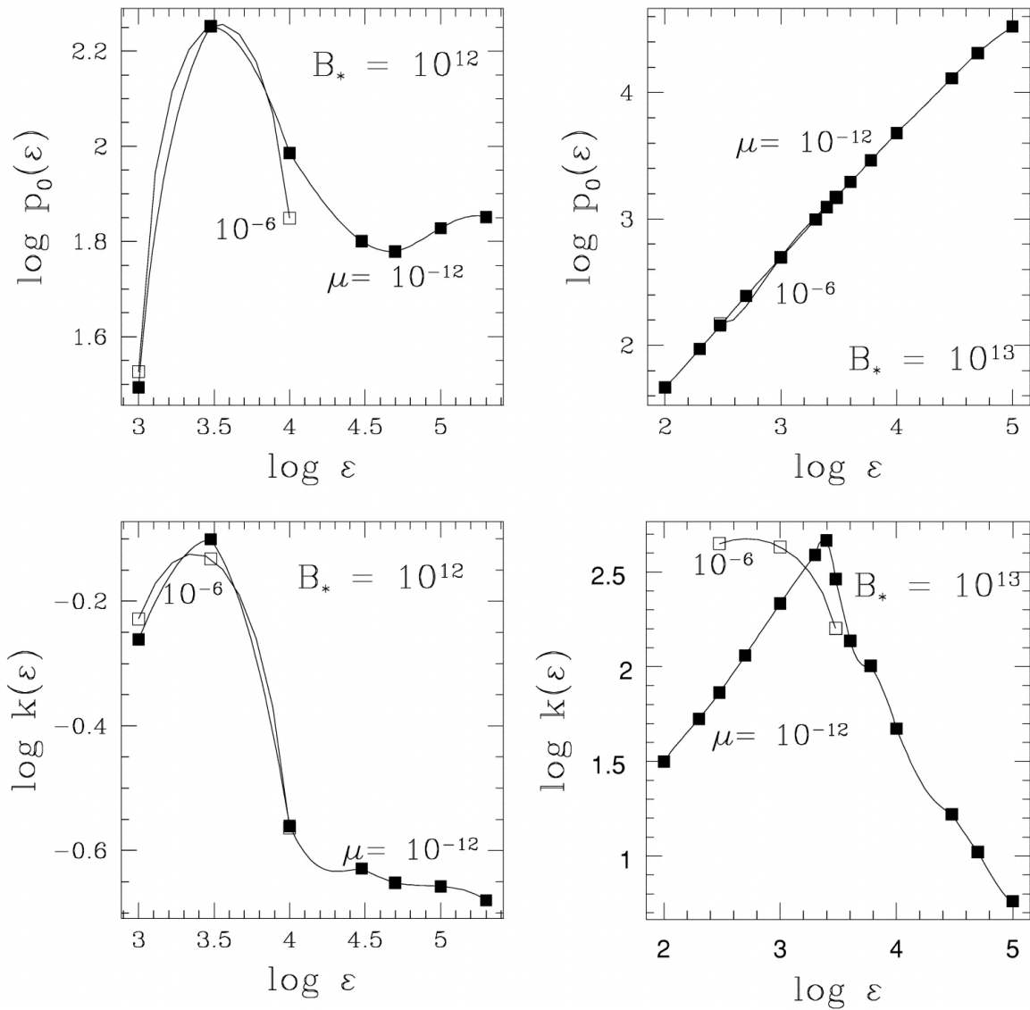
Fig. 5. from Pair Creation in the Pulsar Magnetosphere Arendt & Eilek 2002 ApJ 581 451 doi:10.1086/344133 https://dx.doi.org/10.1086/344133 © 2002. The American Astronomical Society. All rights reserved. Printed in U.S.A.
