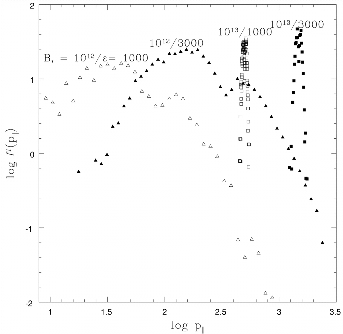
Fig. 4. from Pair Creation in the Pulsar Magnetosphere Arendt & Eilek 2002 ApJ 581 451 doi:10.1086/344133 https://dx.doi.org/10.1086/344133 © 2002. The American Astronomical Society. All rights reserved. Printed in U.S.A.
