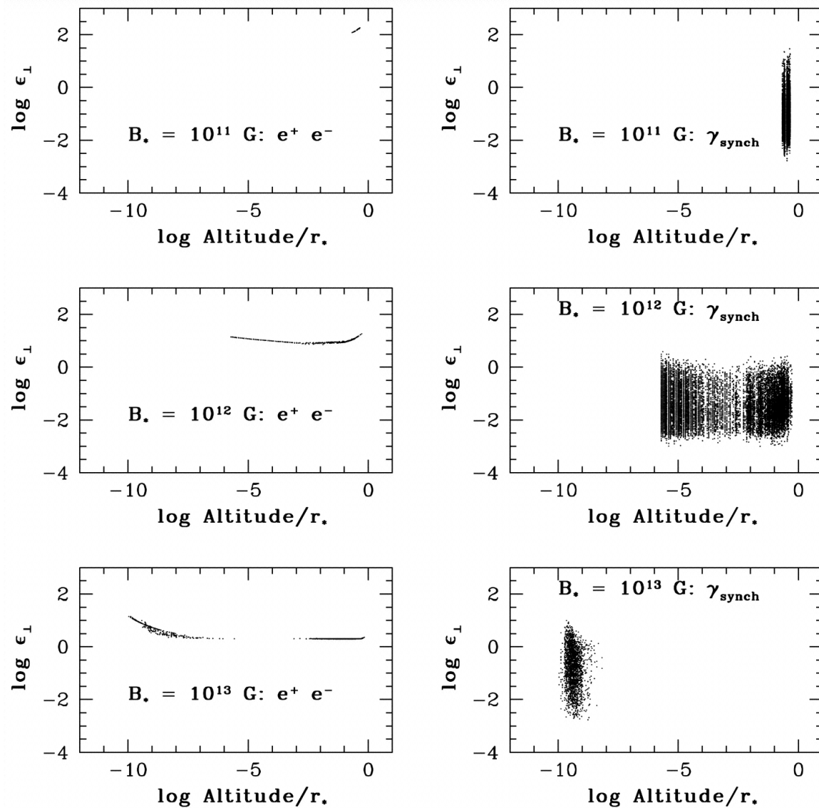
Fig. 2. from Pair Creation in the Pulsar Magnetosphere Arendt & Eilek 2002 ApJ 581 451 doi:10.1086/344133 https://dx.doi.org/10.1086/344133 © 2002. The American Astronomical Society. All rights reserved. Printed in U.S.A.
